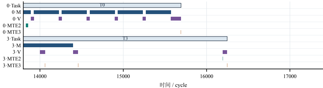
(a) 局部放大 13,800–17,400 cycle · C0:T0, C3:T3
