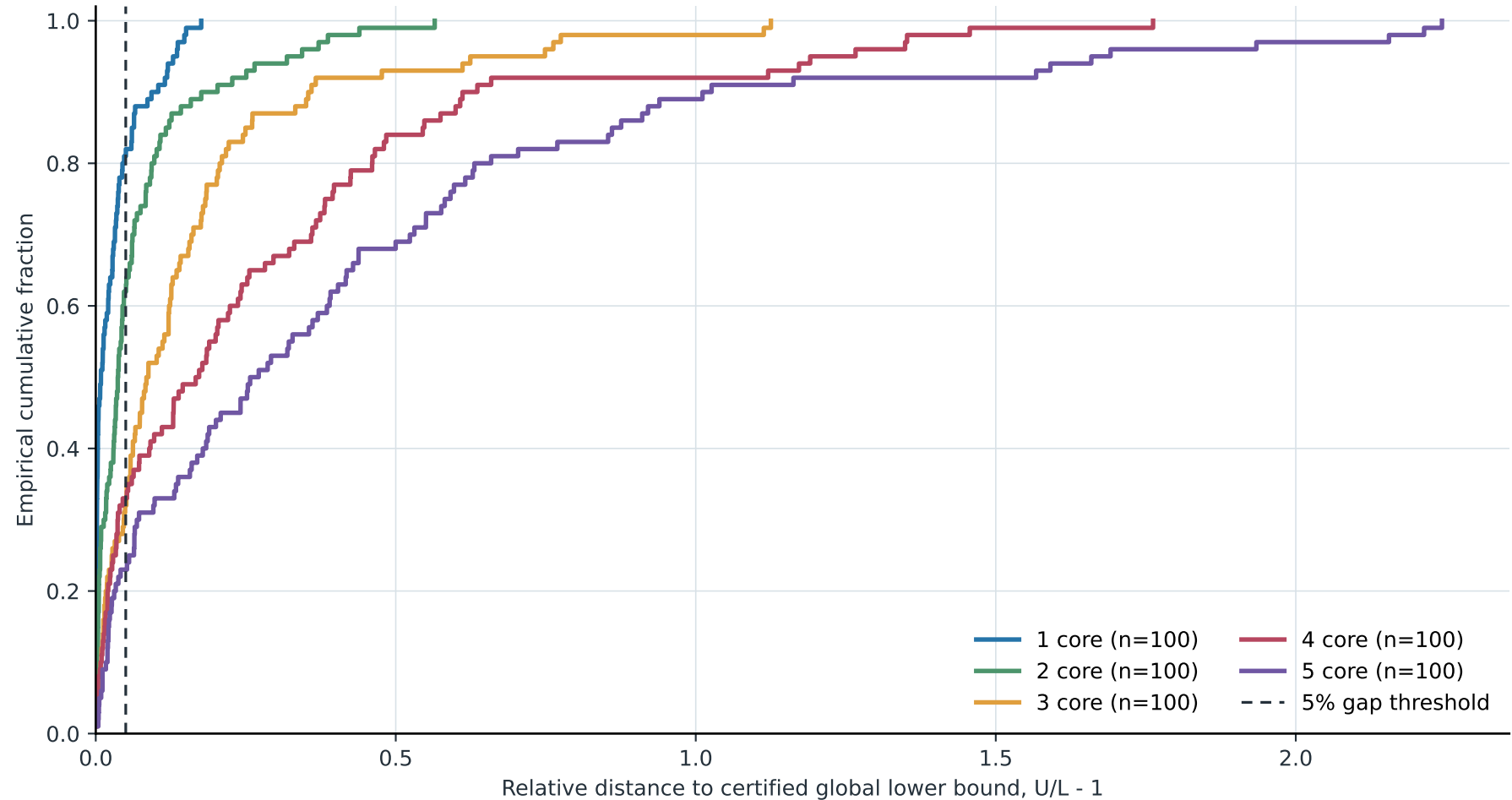
Figure 5-6 | Global lower-bound gap distribution
