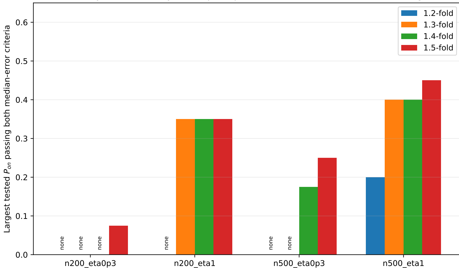
Direct PhysInfer recovery envelope depends on tolerance and observation regime
