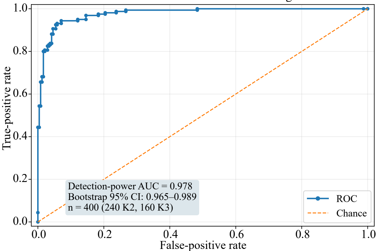
A ROC of effective K2/K3 ranking
