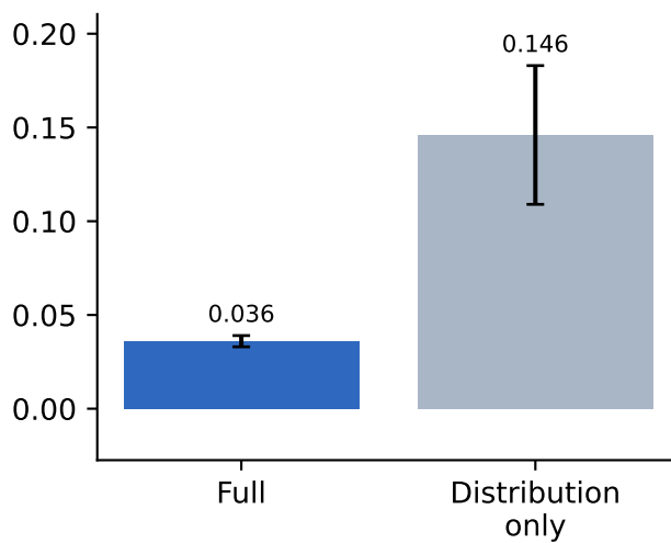
Standardized-distribution W1
