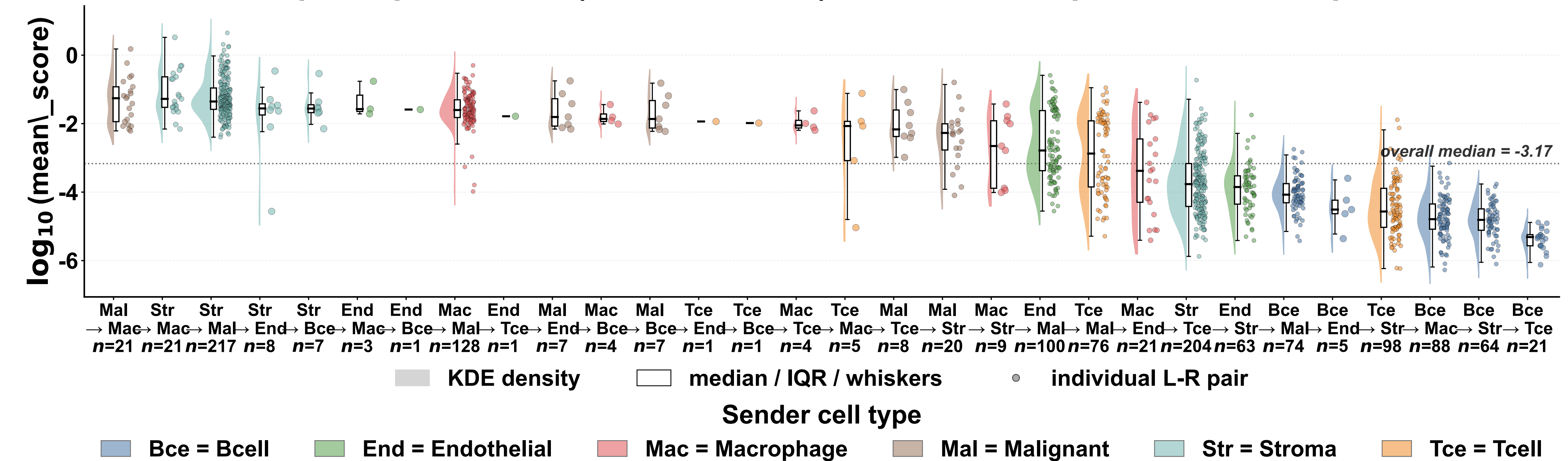
A. Spatial prior score (BreastCancer2) — N=1287 L-R pairs, 30 cluster pairs
