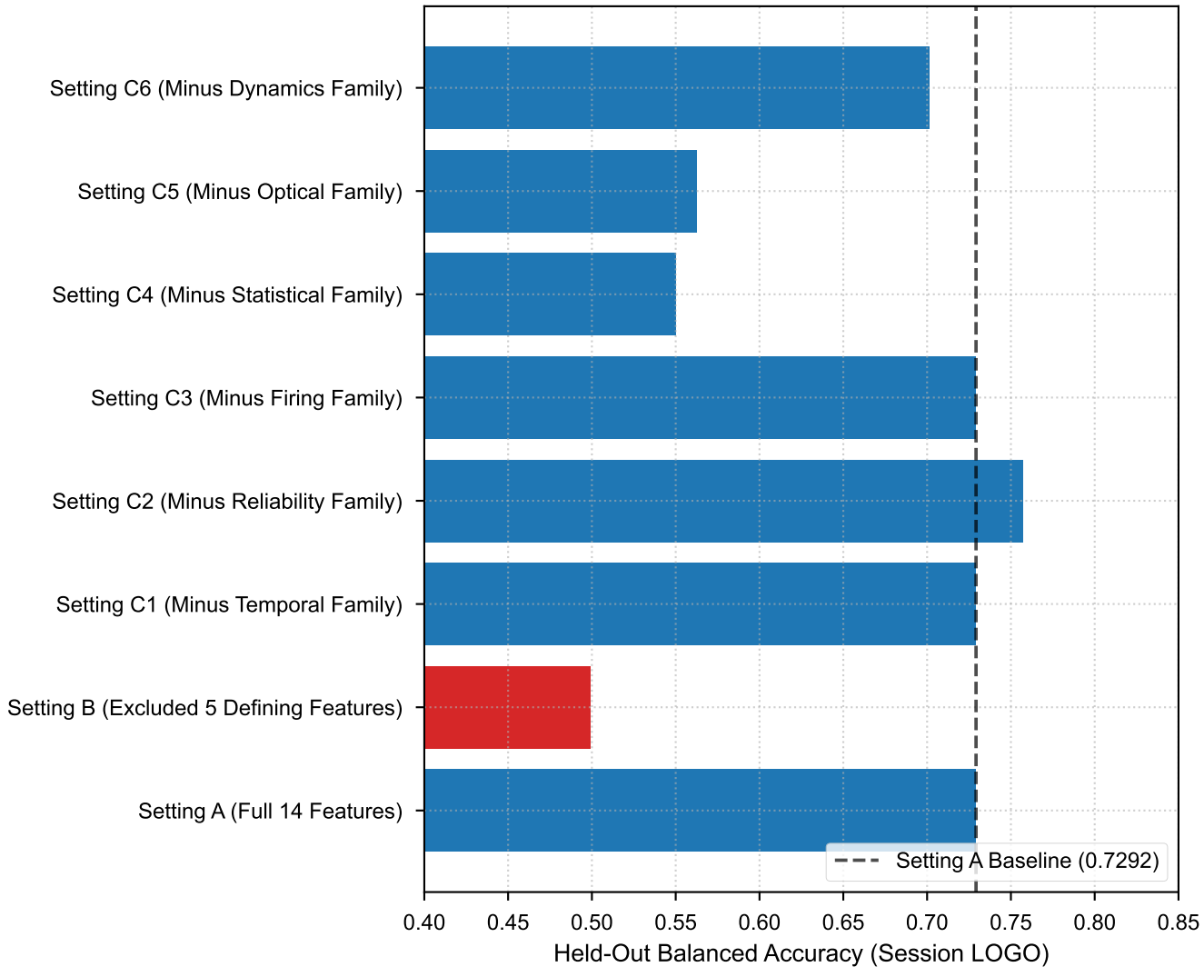
A. Label Circularity: Collapse When Defining Features are Excluded
