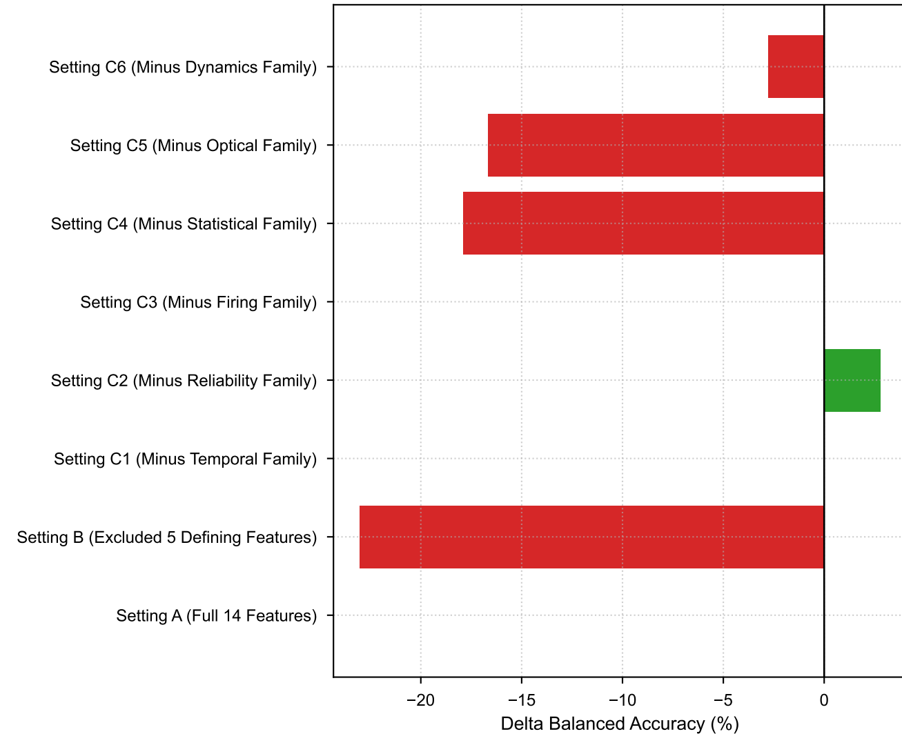
B. Performance Delta Relative to Setting A (% Points)
