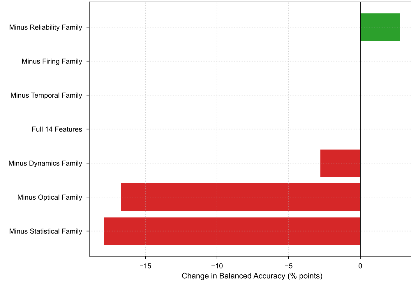
A. Feature-Family Criticality Ranking ( \Delta Balanced Accuracy %)
