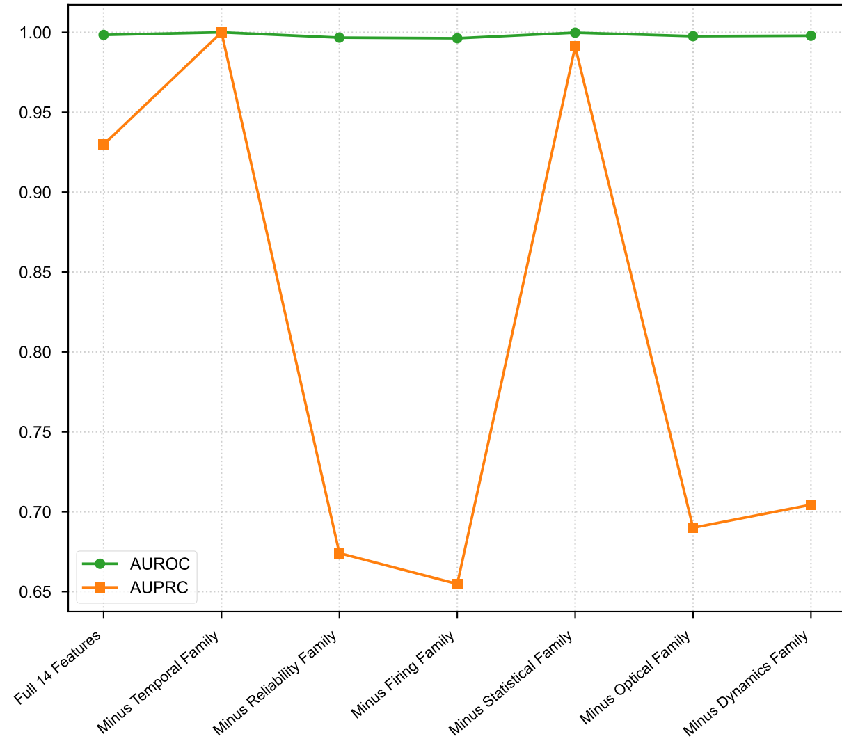
B. AUROC vs AUPRC Under Feature Family Ablation
