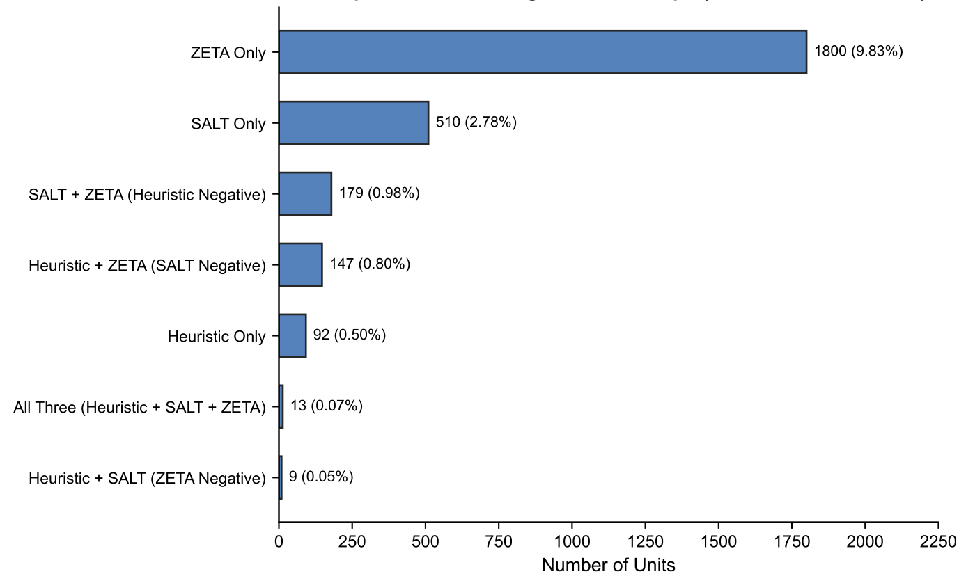
A. Responsiveness Disagreement Groups (Heuristic, SALT, ZETA)
