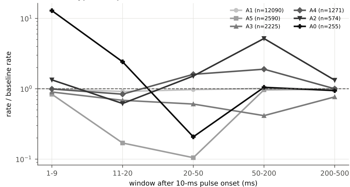
A Archetype rate profiles (multinomial mixture)
