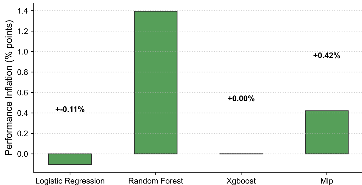
B. Quantified Intra-Recording Leakage Inflation ( \Delta BA)
