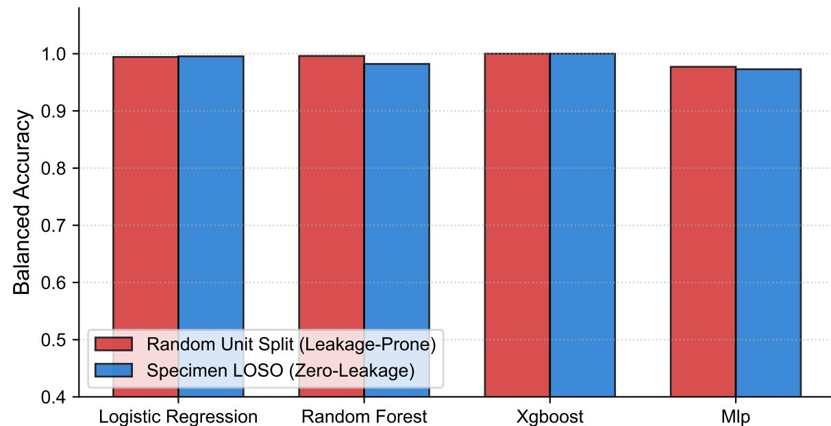
A. Balanced Accuracy across Validation Regimes
