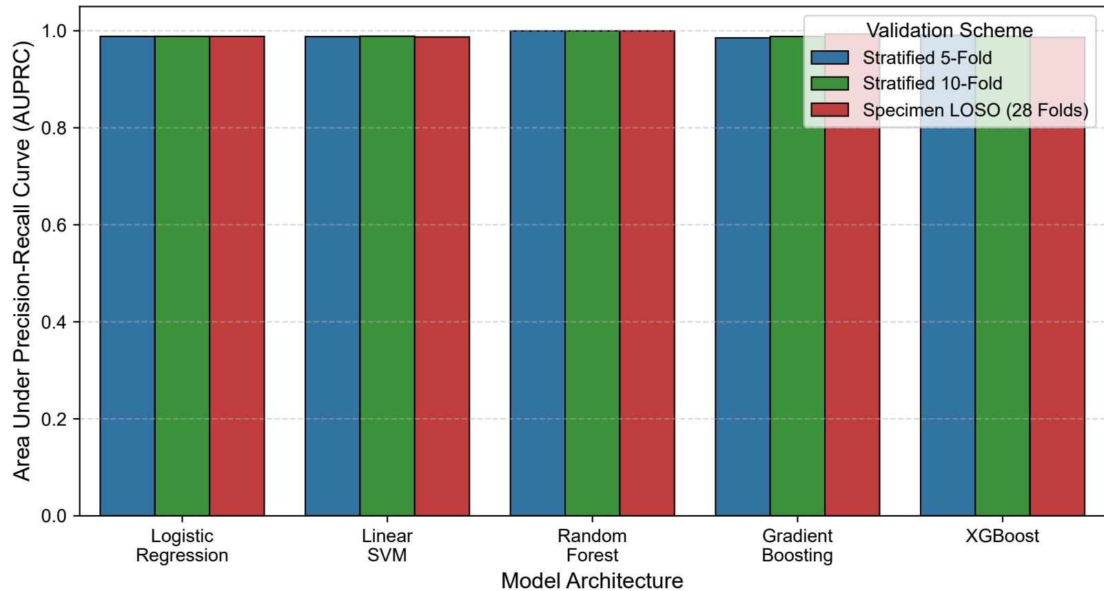
Figure Audit 1: Validation Scheme Comparison (Stratified K-Fold vs Specimen LOSO)
