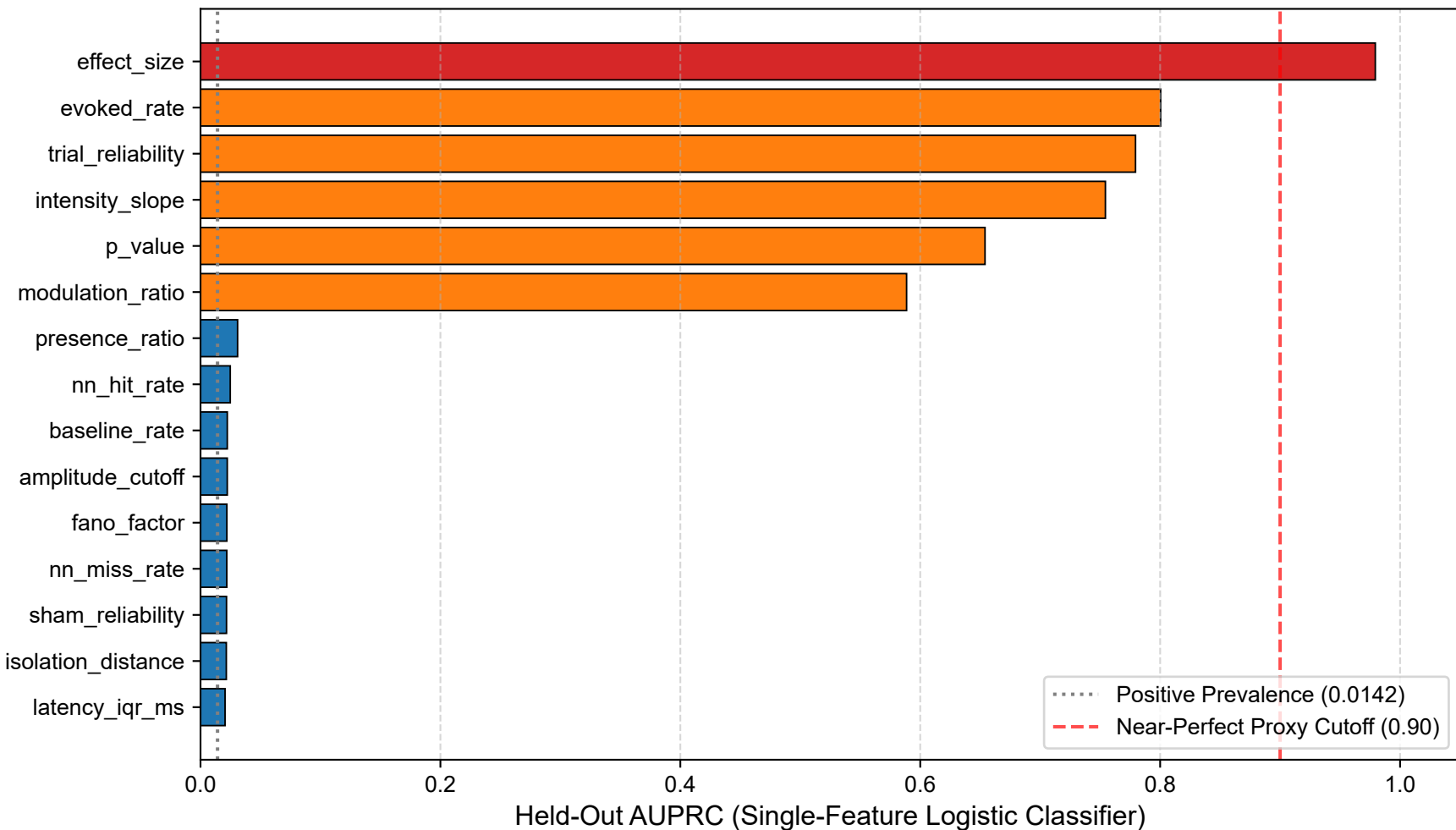
Figure Audit 3: Univariate Predictive Strength (Specimen LOSO AUPRC)
