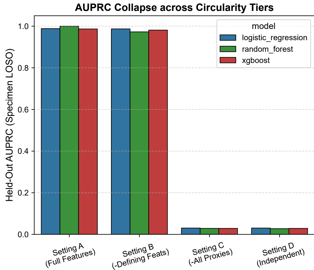
Figure Audit 4: Systematic Deconstruction of Label Circularity (Settings A, B, C, D)
