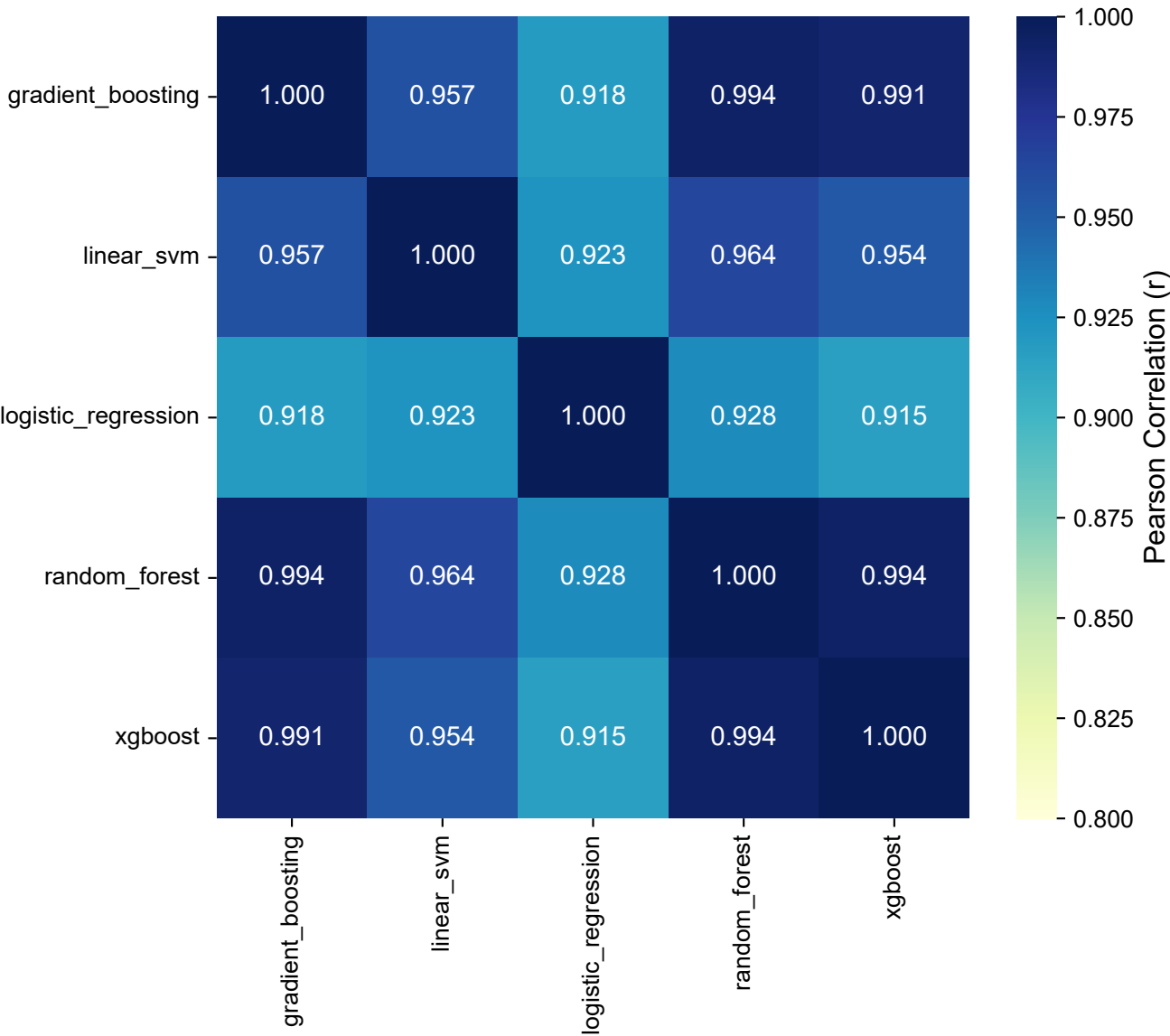
Figure Audit 7: Pairwise Prediction Correlation across Models
