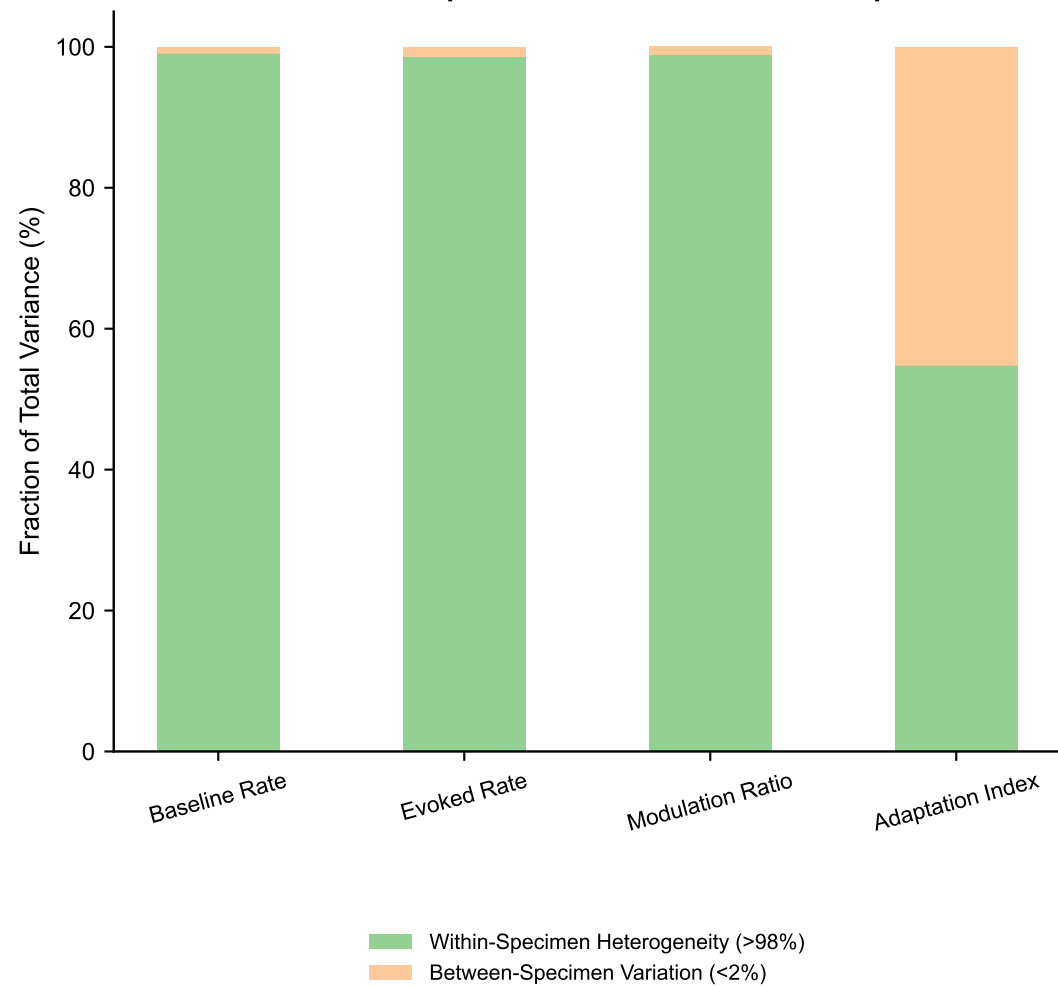
B. Variance Decomposition: Within vs. Between Specimen
