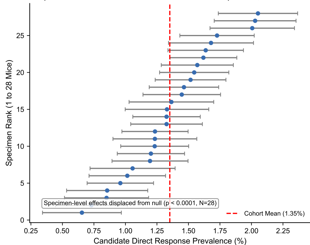
A. Specimen-Level Direct Candidate Prevalence (95% CI, N = 28 Mice)
