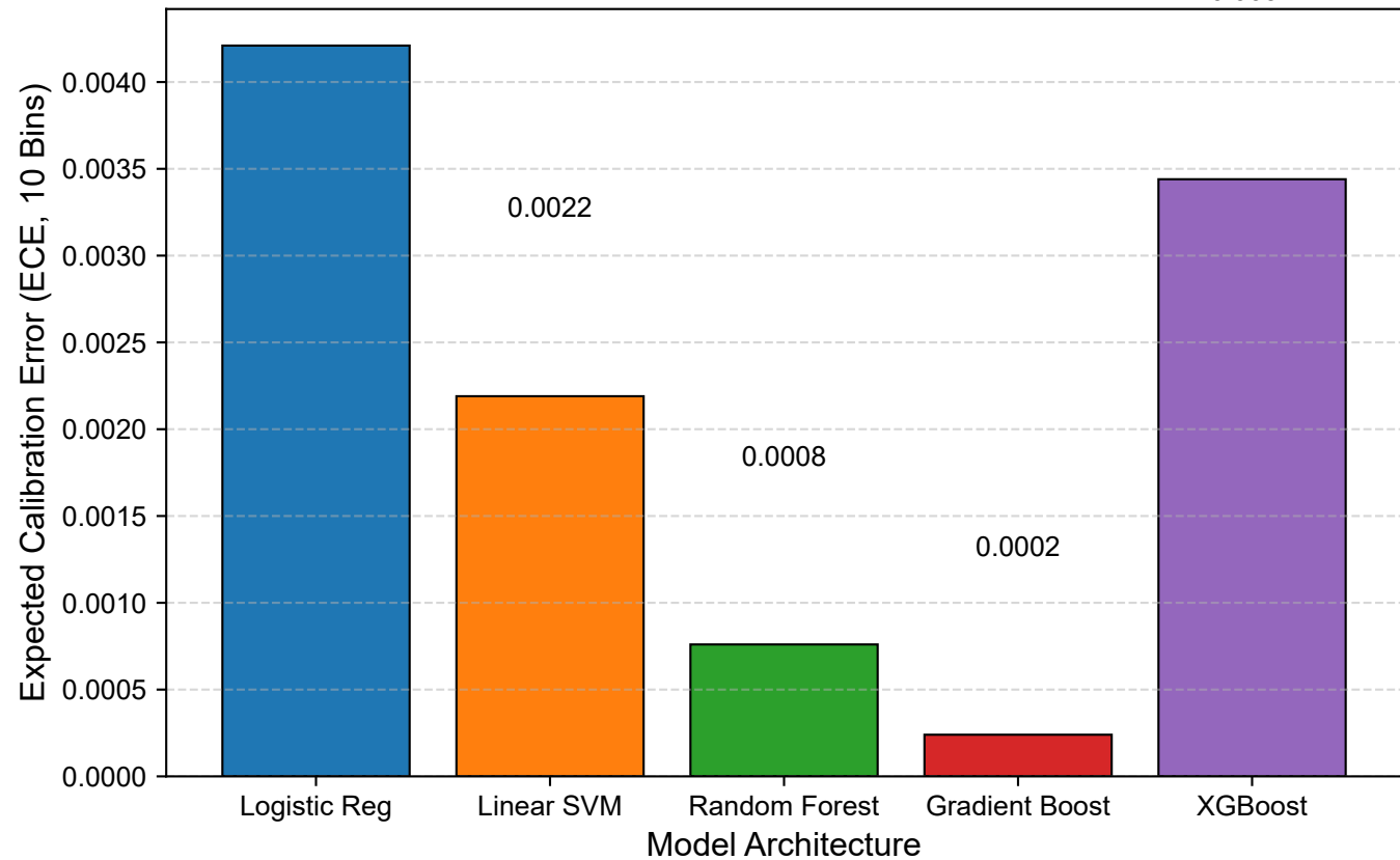
Figure Audit 5: Expected Calibration Error (ECE) across Models
