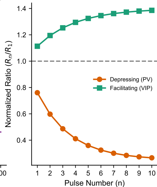
E. 10-Hz Train Dynamics (Normalized Response R_n/R_1 )
