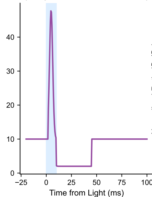
D. Biphasic Dynamics (Early Burst → Circuit Pause)
