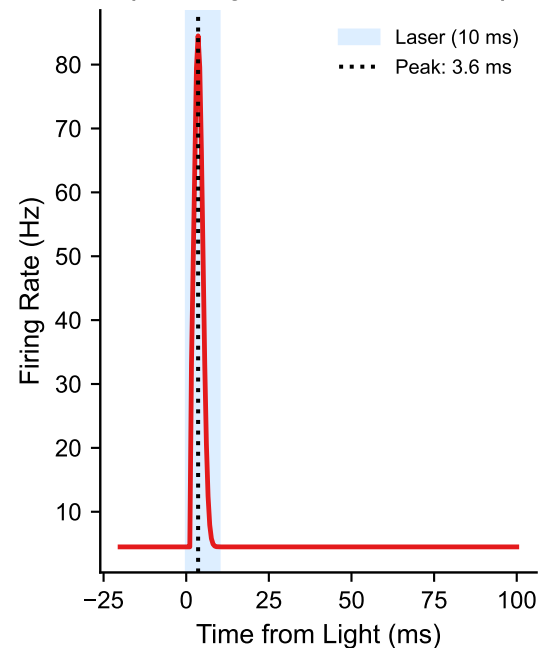
A. Direct-Like Excitation (Latency < 8 ms, Rel = 0.82)
