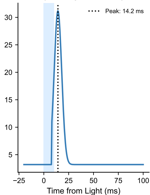
B. Early Network Excitation (Latency = 11.5 ms)
