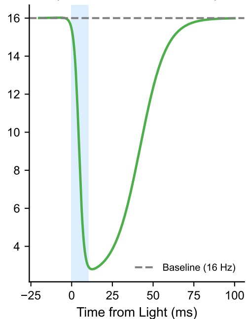
C. Network Suppression (Inhibition W3/W4: 85%)
