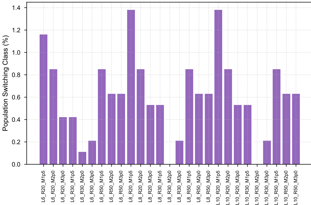
C. Units Changing Operational Class (% Population)
