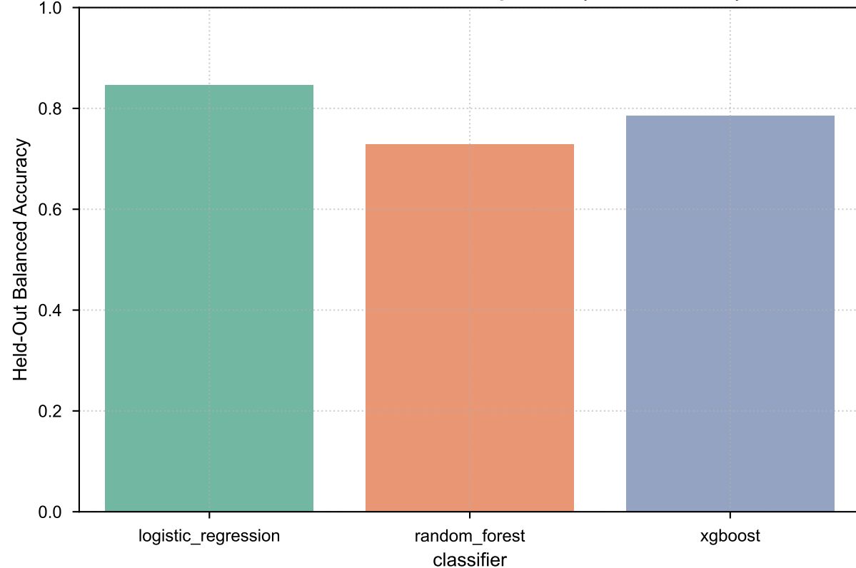
D. Classifier Architecture Comparison (Session LOGO)
