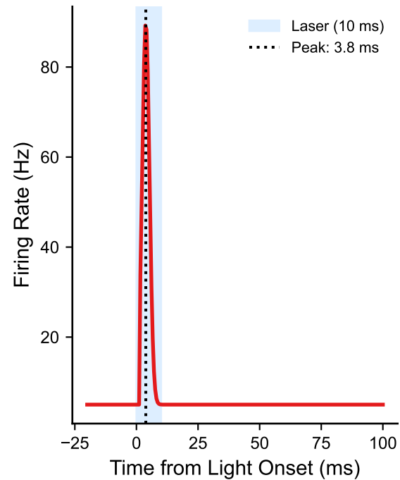
A. Direct Optical Excitation (Latency < 8 ms, Rel = 0.88)
