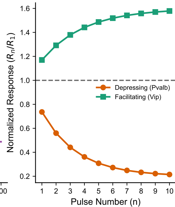
E. 10-Hz Train Adaptation (Pulse n / Pulse 1 Response)
