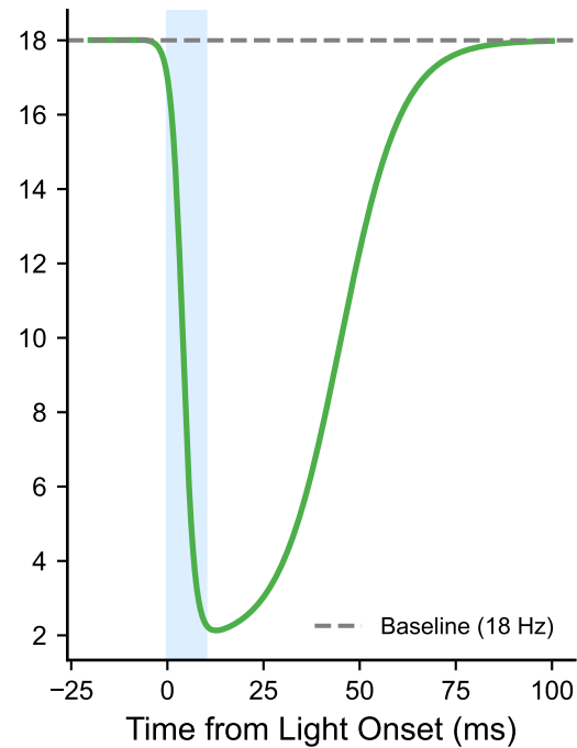
C. Profound Network Suppression (Inhibition W3/W4: 85%)
