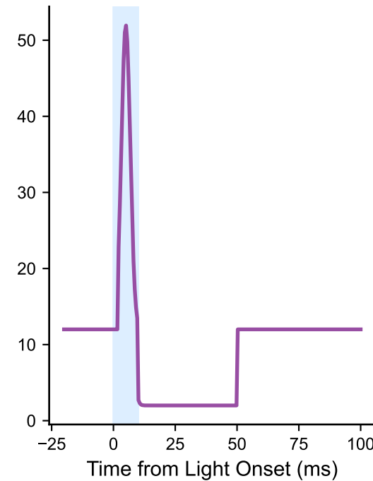
D. Excitation → Suppression (Direct Burst → Circuit Silence)
