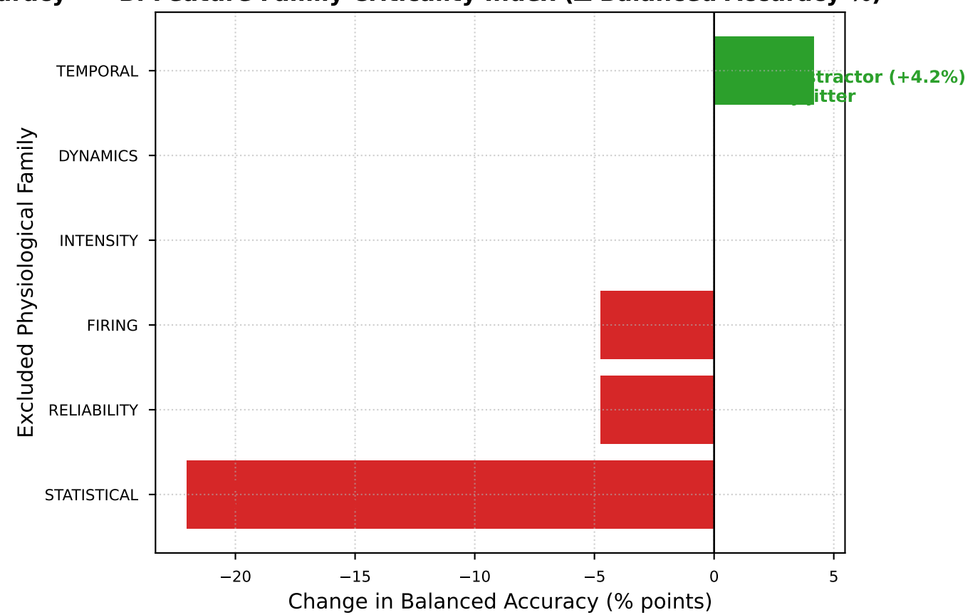
B. Feature Family Criticality Index ( \Delta Balanced Accuracy %)
