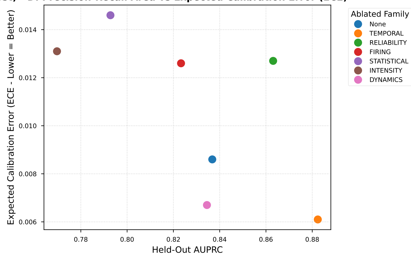
D. Precision-Recall Area vs Expected Calibration Error (ECE)
