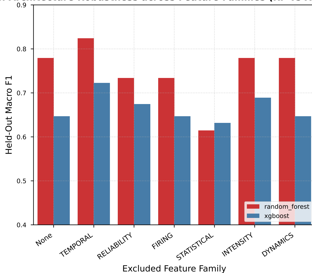
C. Architecture Robustness across Feature Families (RF vs XGBoost)
