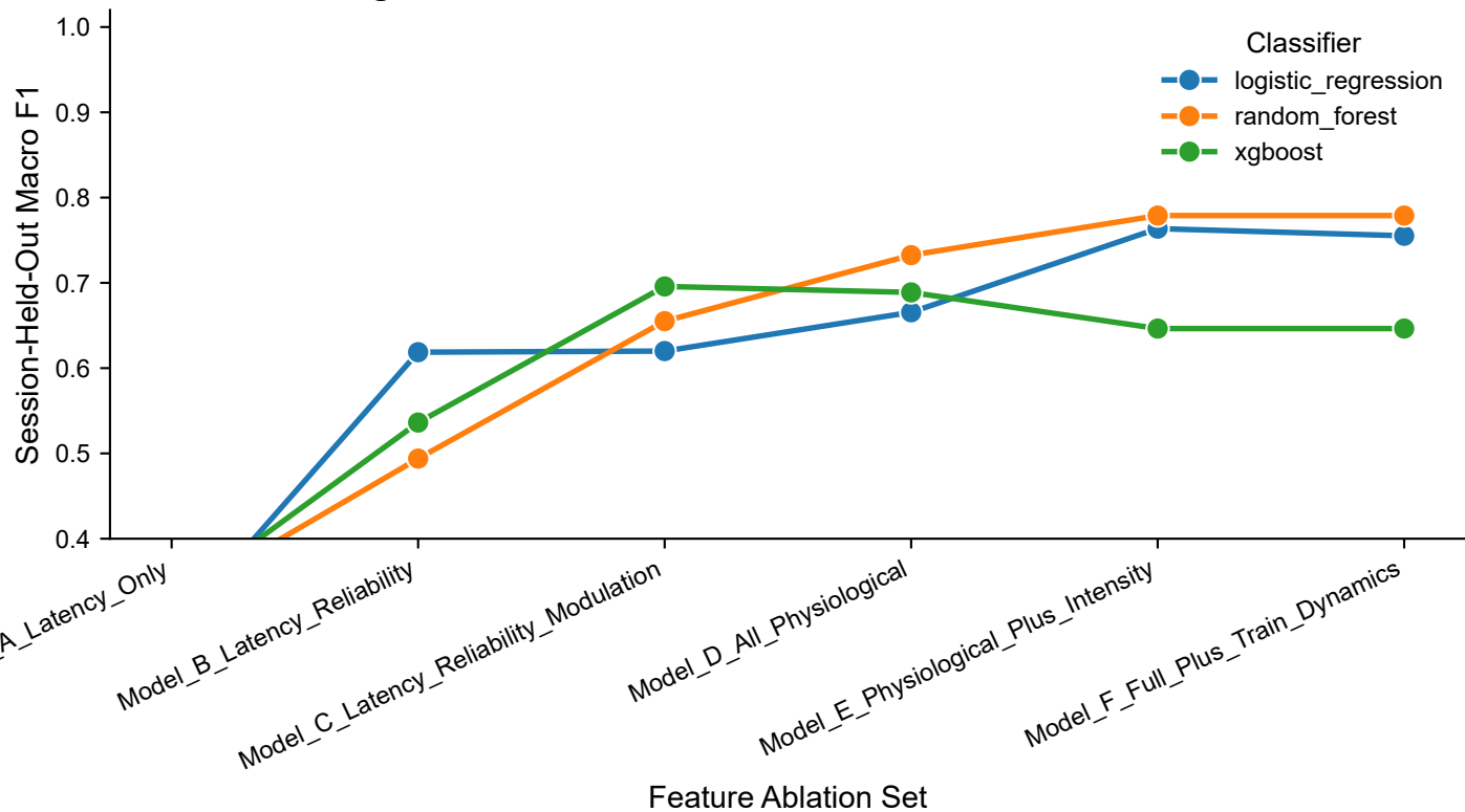
Figure 6: Feature Ablation Contribution to Classification
