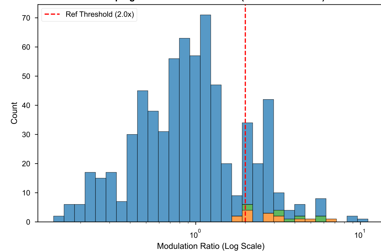
C. Optogenetic Modulation Ratio (Evoked / Baseline)
