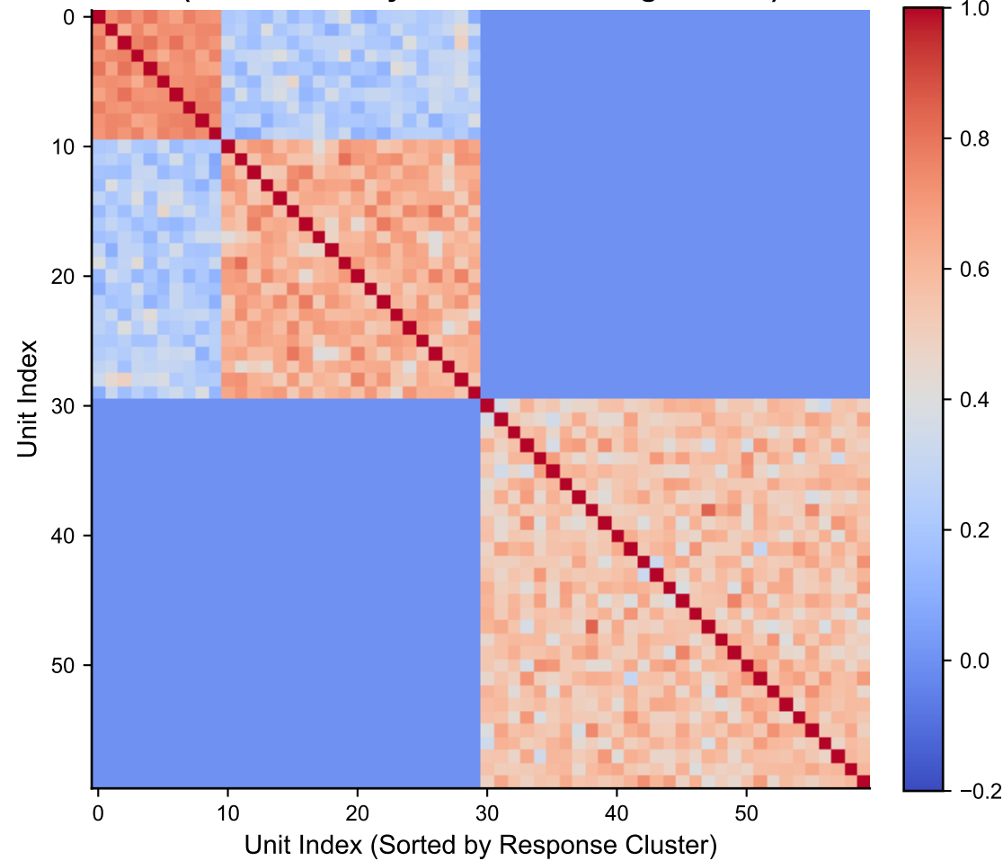
A. Response Correlation Matrix: \text{corr}(R_i(t), R_j(t)) (Simultaneously Recorded on Single Probe)
