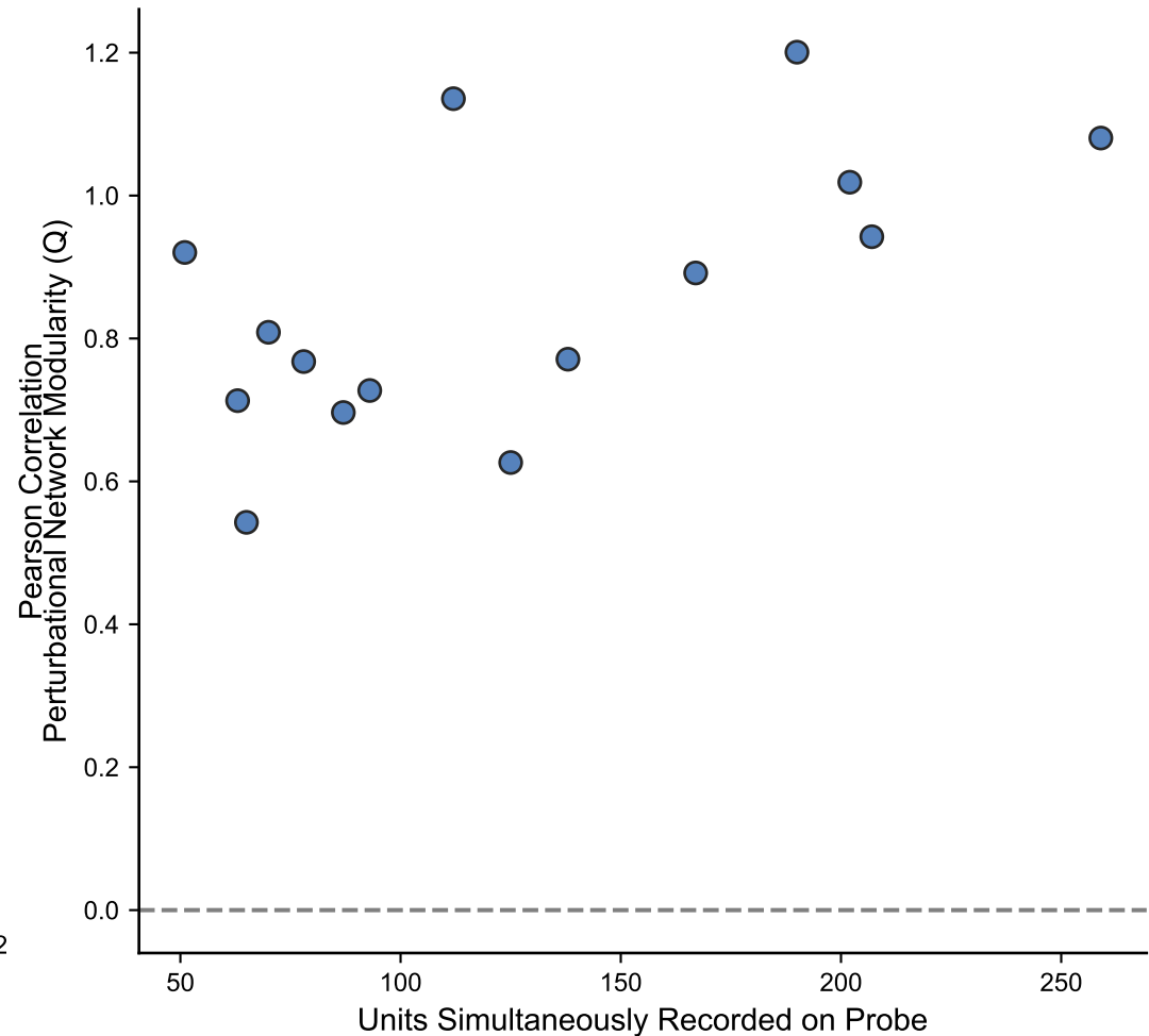
B. Functional Clustering Beyond Physical Proximity
