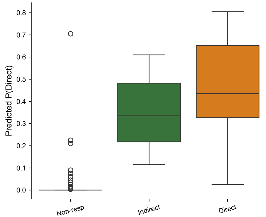
A. Direct Class Probability Assignment
