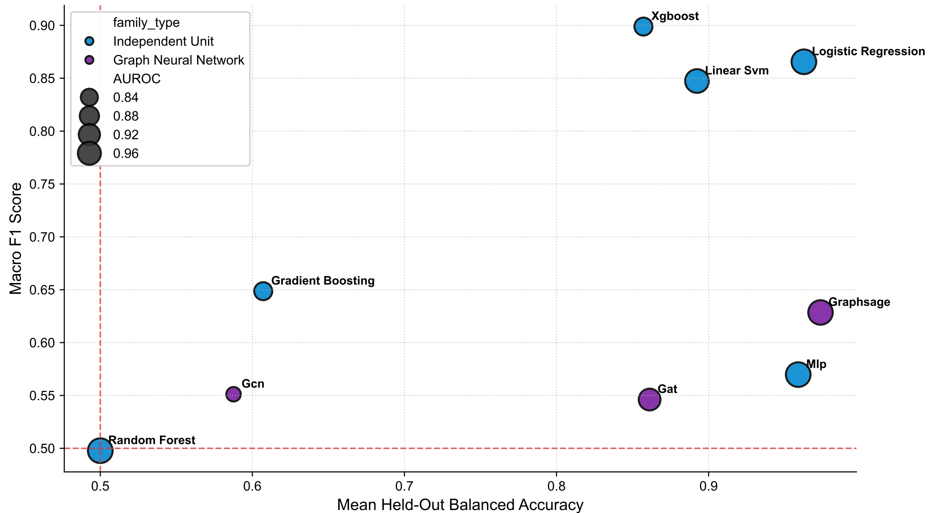
Figure ML5: Graph Neural Networks vs Independent-Unit Physiological Baselines
