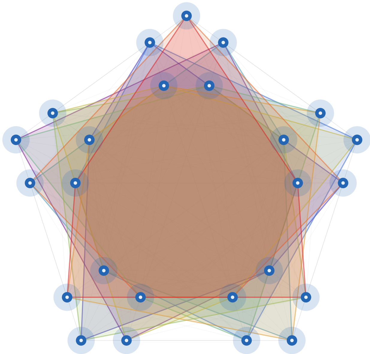
GE exclusivity hypergraph C_5(OR) \otimes C_5 (25 events, 200 exclusivity edges, 10 pentad hyperedges)
