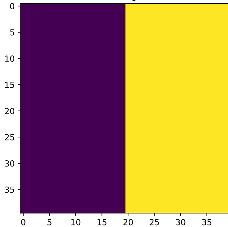
True g_{11}
