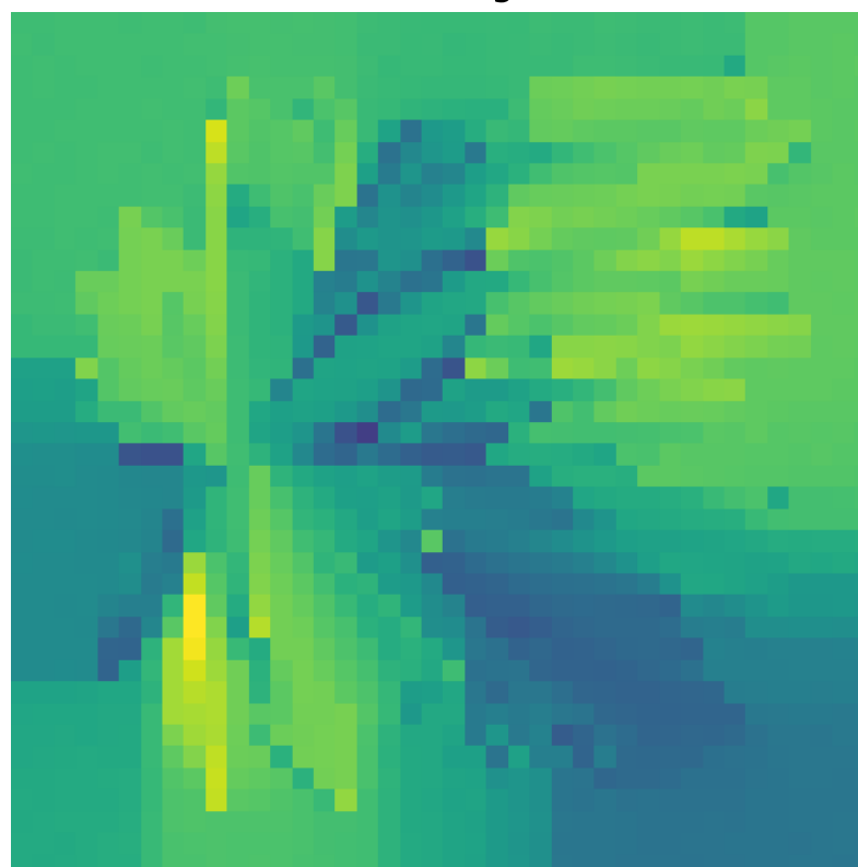
Eikonal g_{22}
