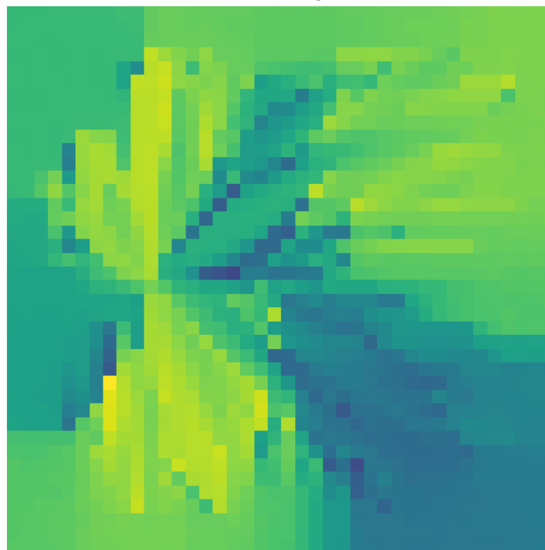
Eikonal g_{12}
