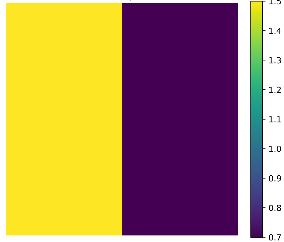
True g_{11}
