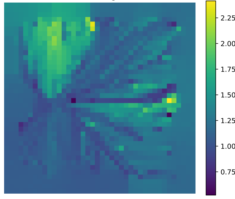
Eikonal g_{11}
