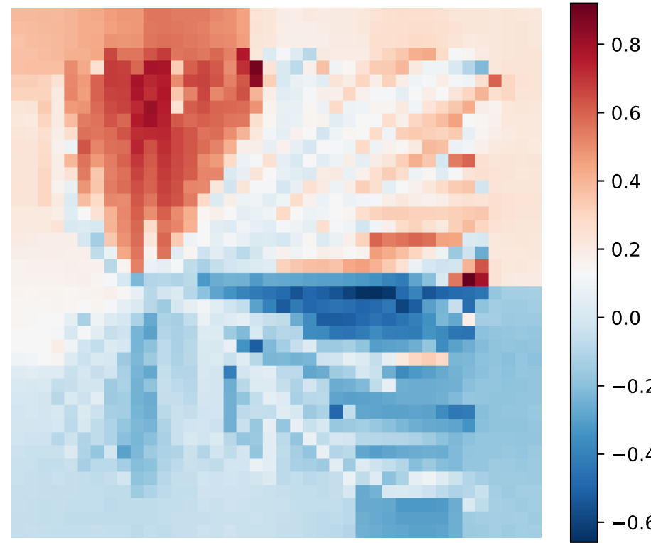
Eikonal b_1
