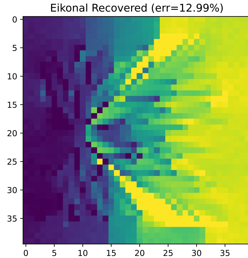
C2: Sparse Recovery (10% obs)
