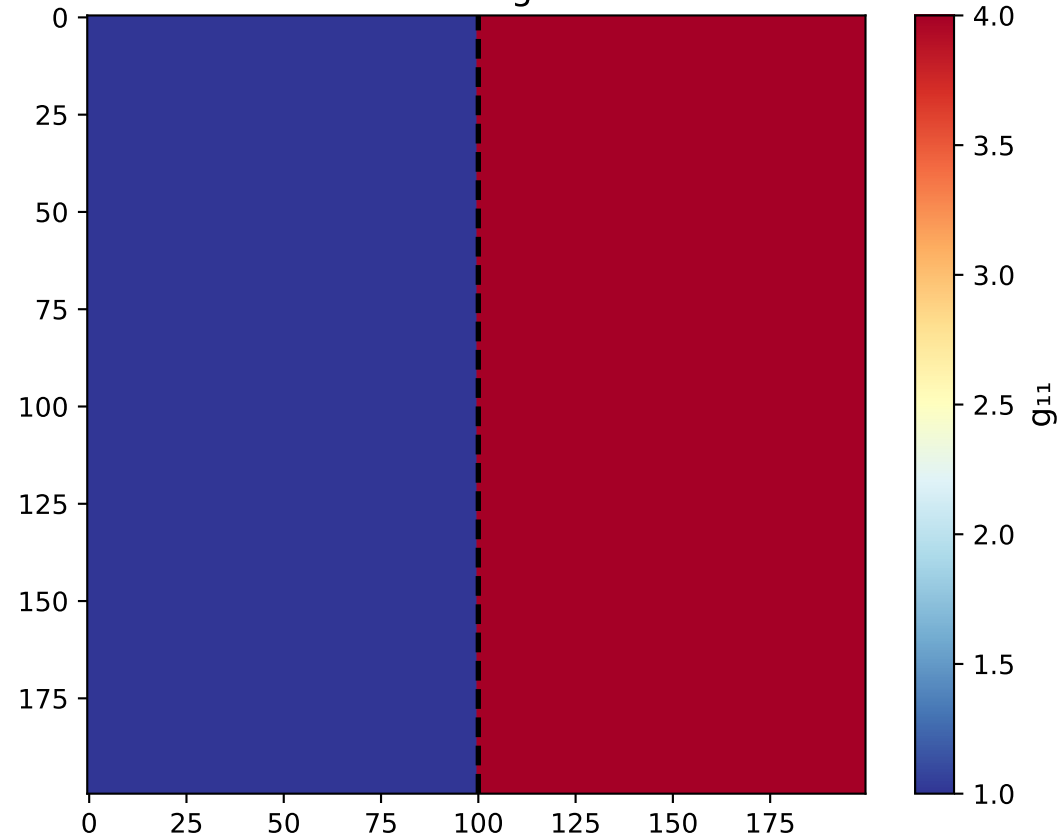
Metric g_{11}
