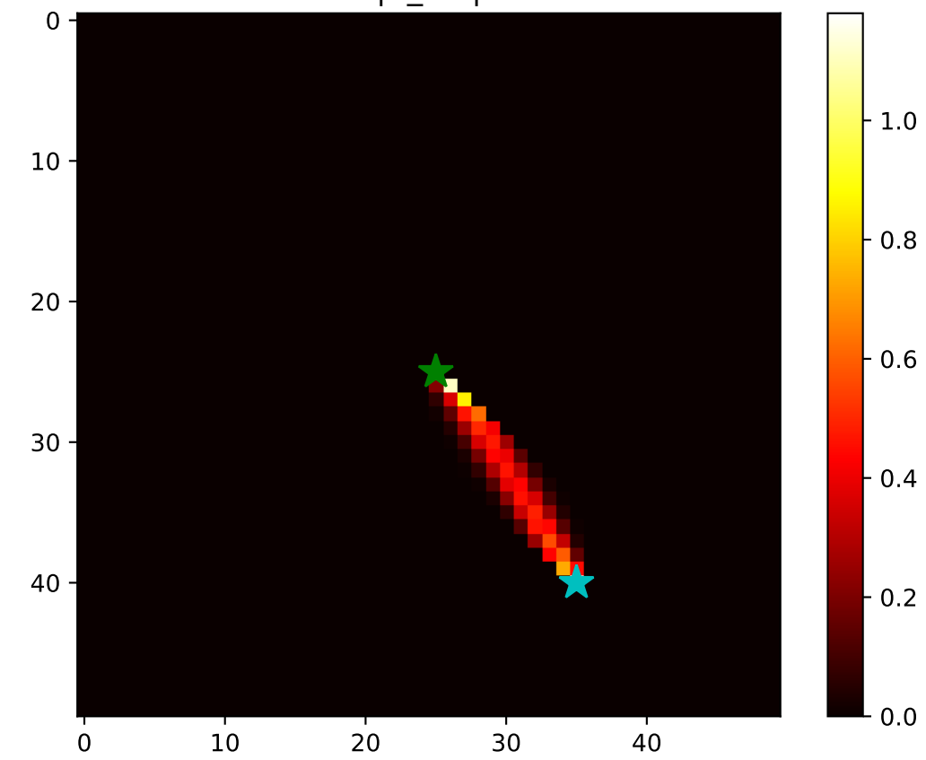
|\nabla_B L|
