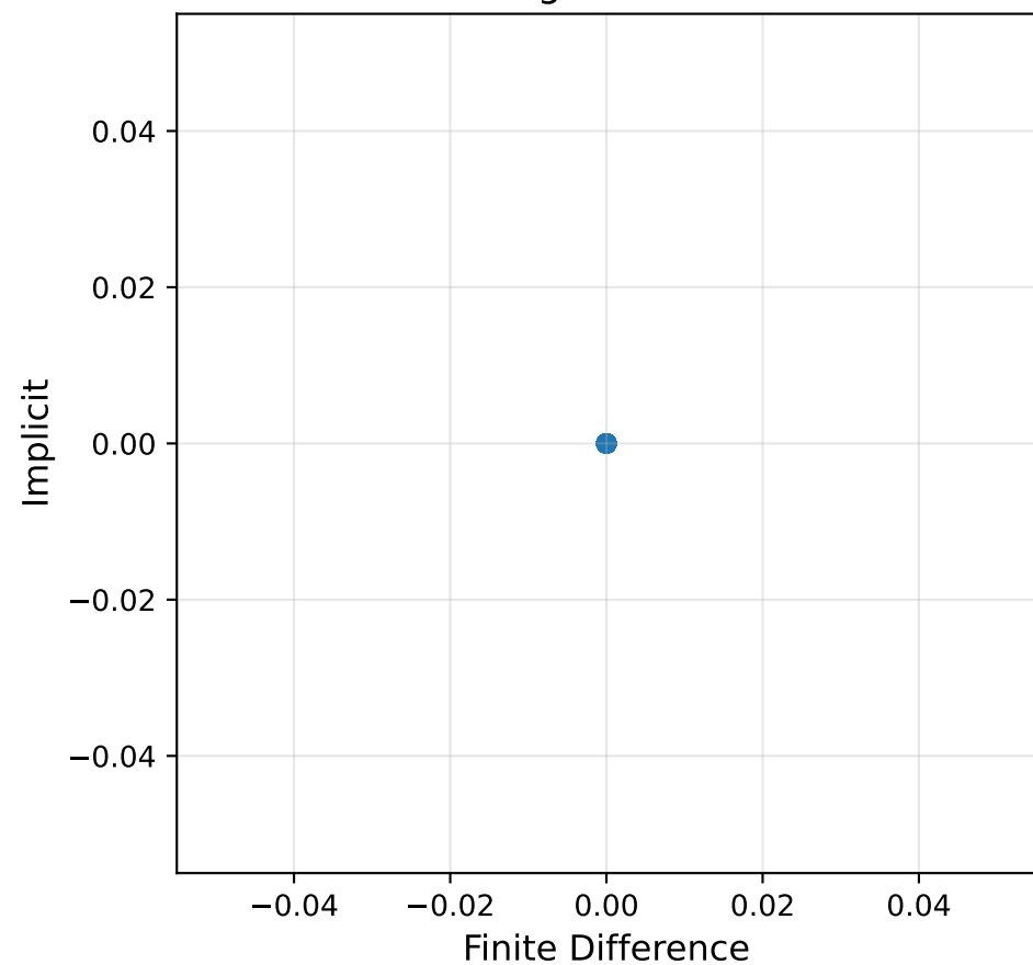
|\nabla_B L|
