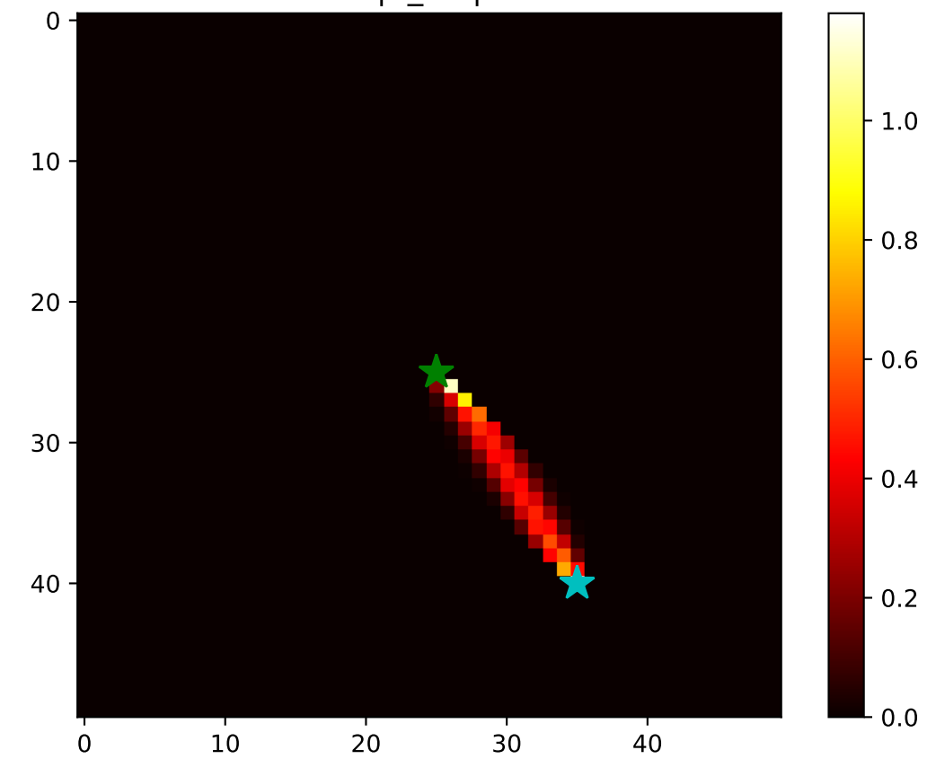
|\nabla_B L|
