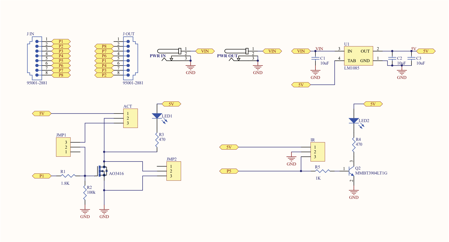
2 Jackplate Schematic
