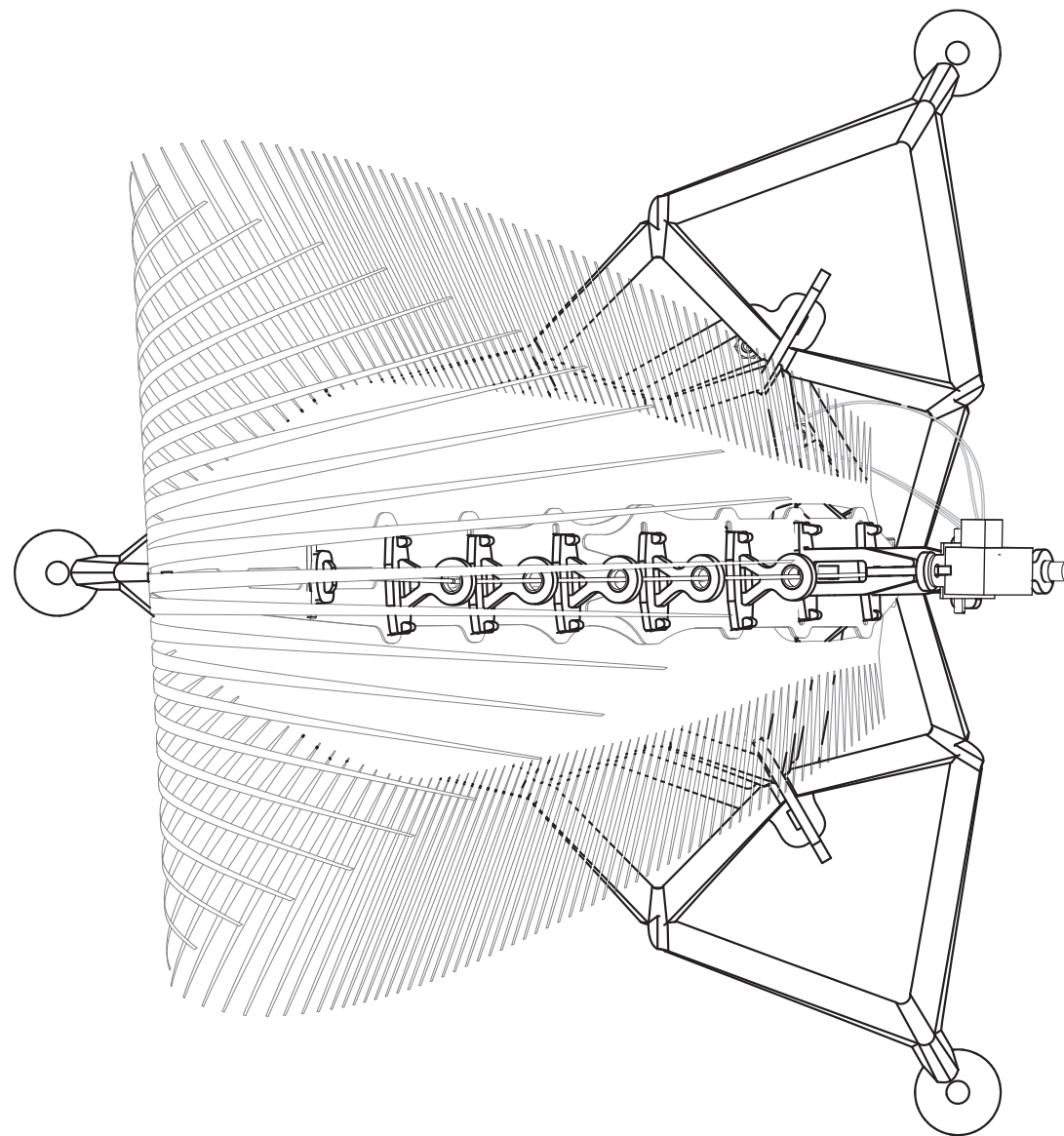
2 Plan (Top View)
