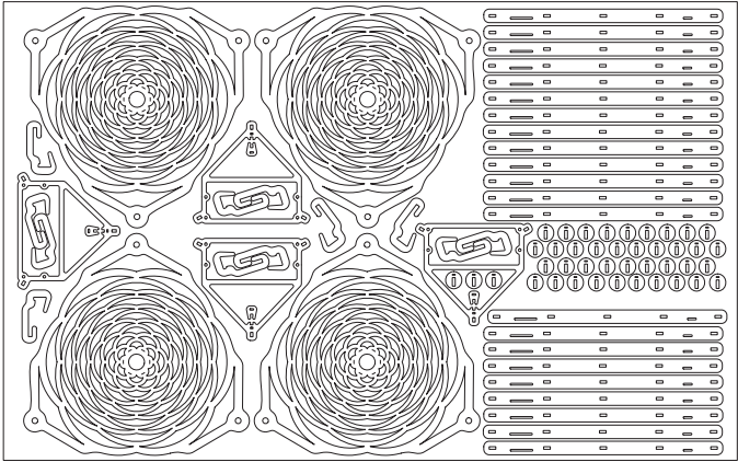
3mm Acrylic x 1
