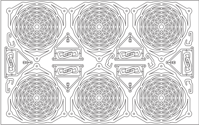
3mm Acrylic x 6
