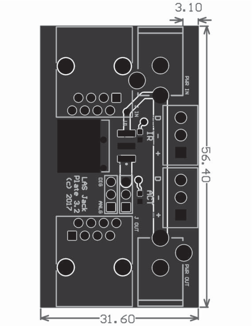
1 Jackplate Detail
