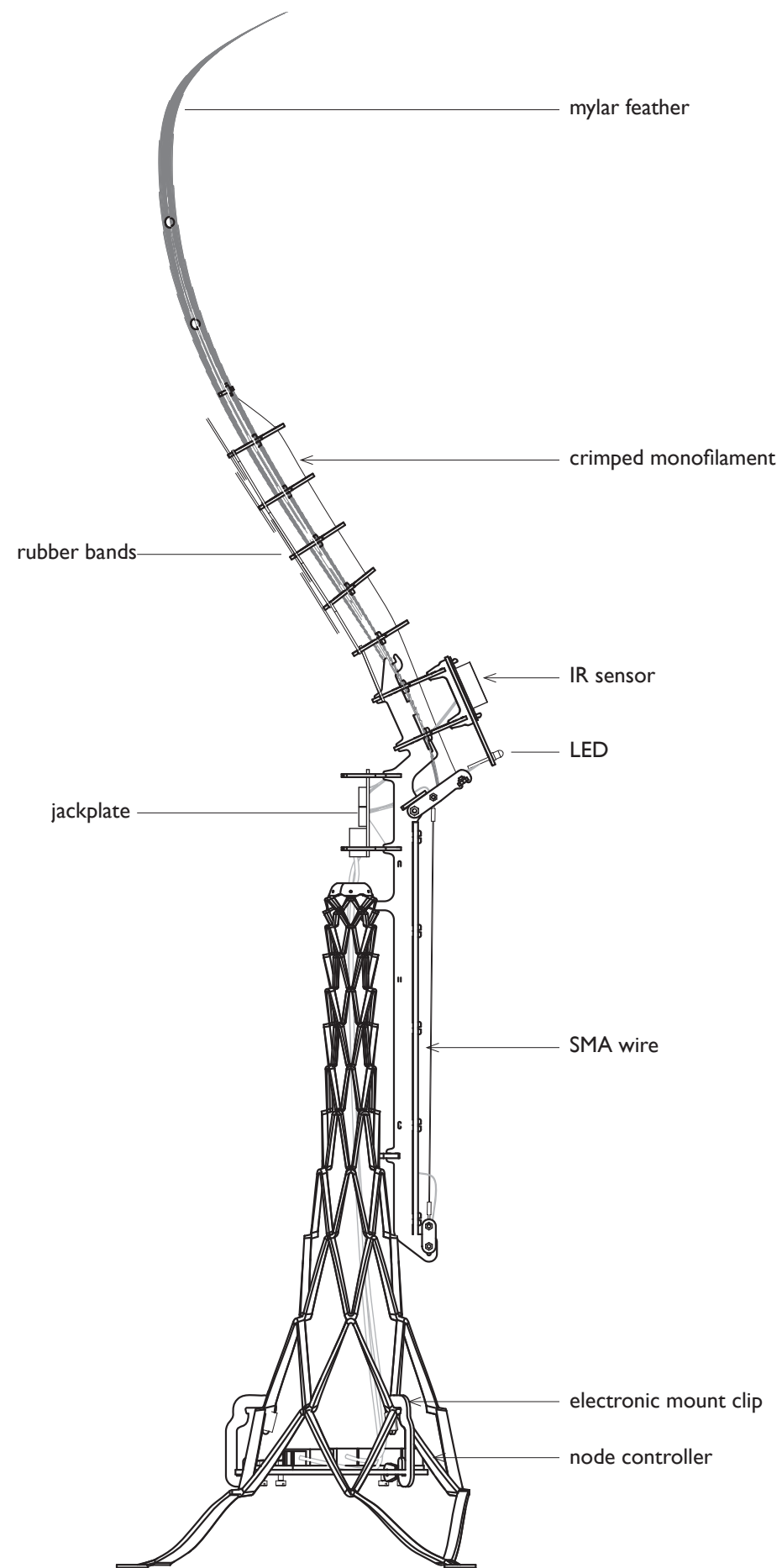
1 Elevation (Side View)
