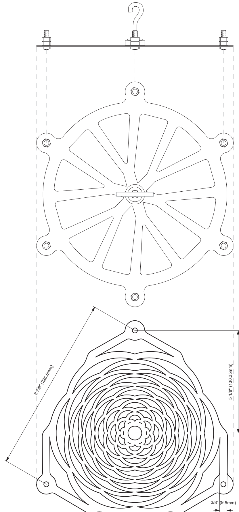
2 Cutting Pattern and Forming Plate 3mm Acrylic Fastened to Steel Frame
