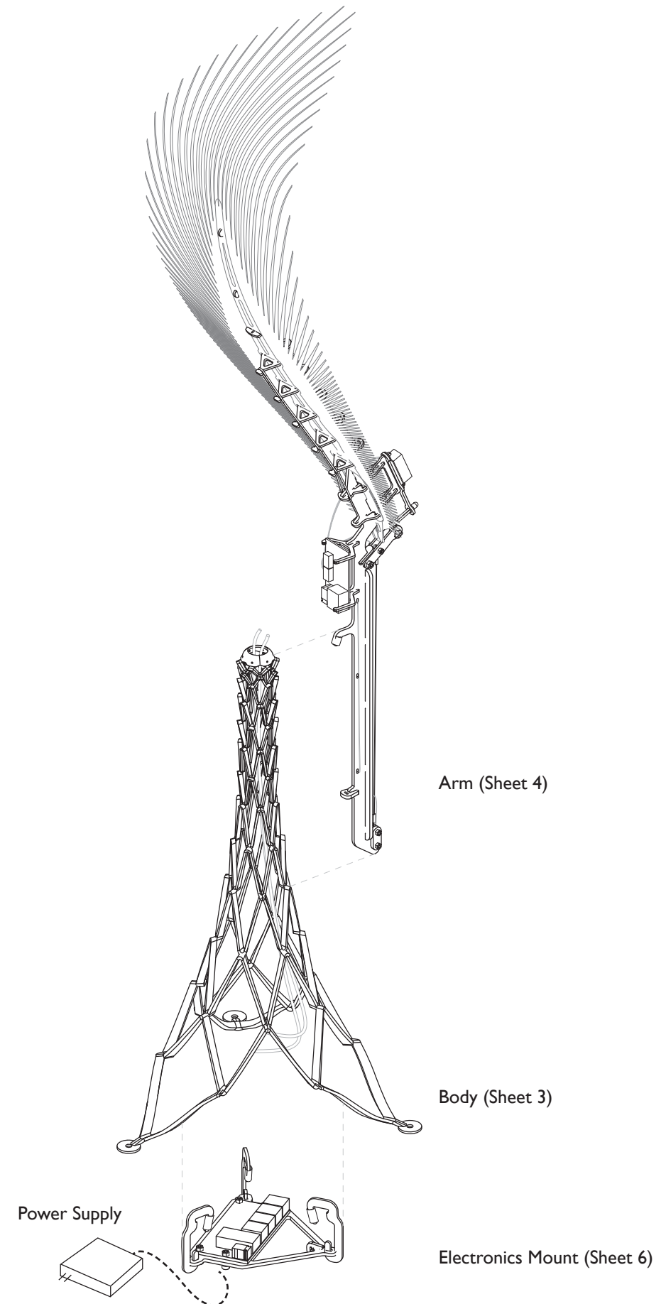
3 Assembly Drawing
