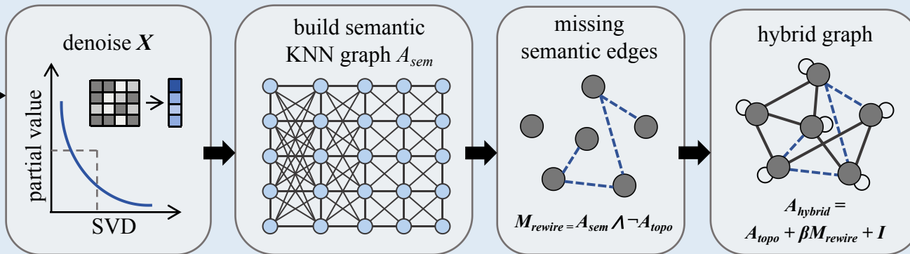
(B) Complementary Semantic Route Construction
