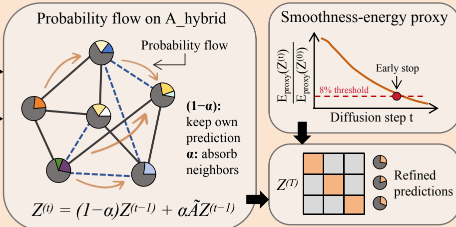
(C) Smoothness-Controlled Diffusion
