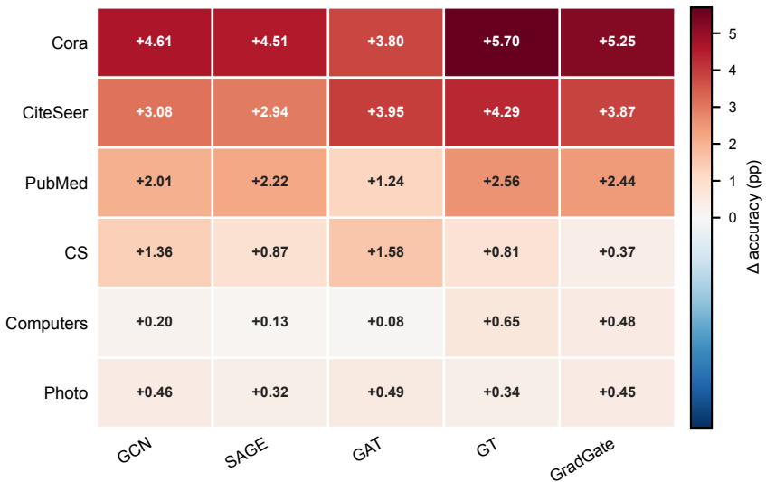
A. Accuracy gain after SETTA
