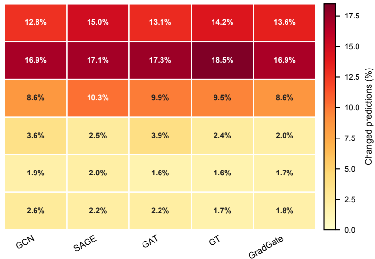
B. Test predictions changed
