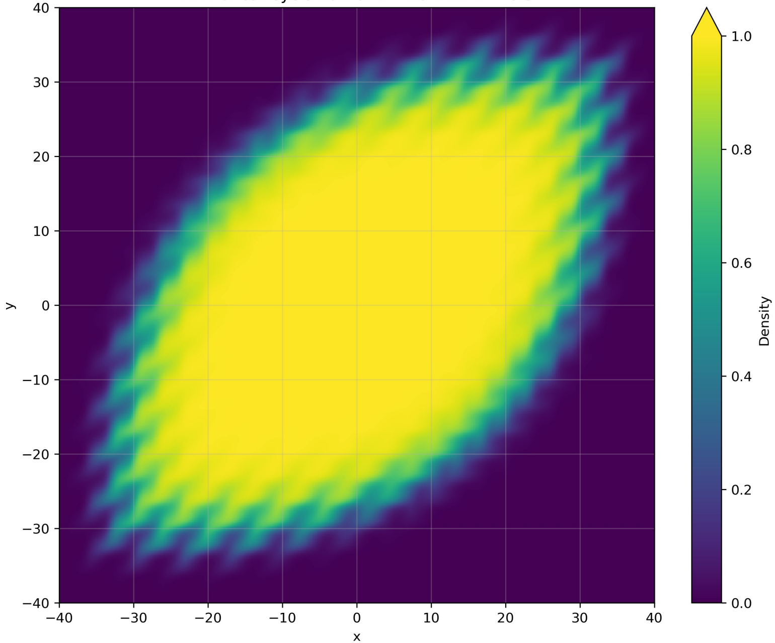
FDM of cat eye's flow at t = 20 with D = 0.5
