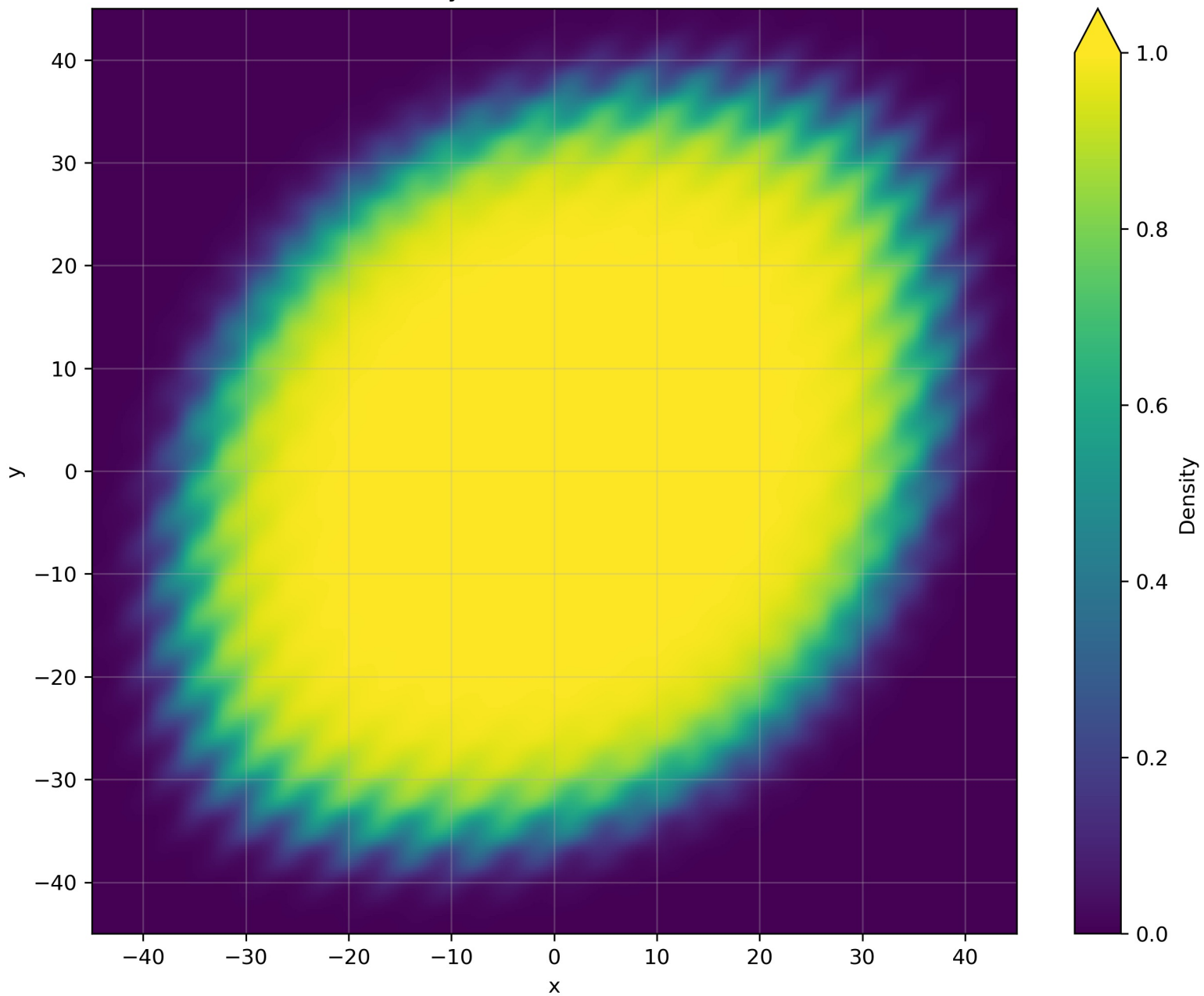
FDM of cat eye's flow at t = 20 with D = 1
