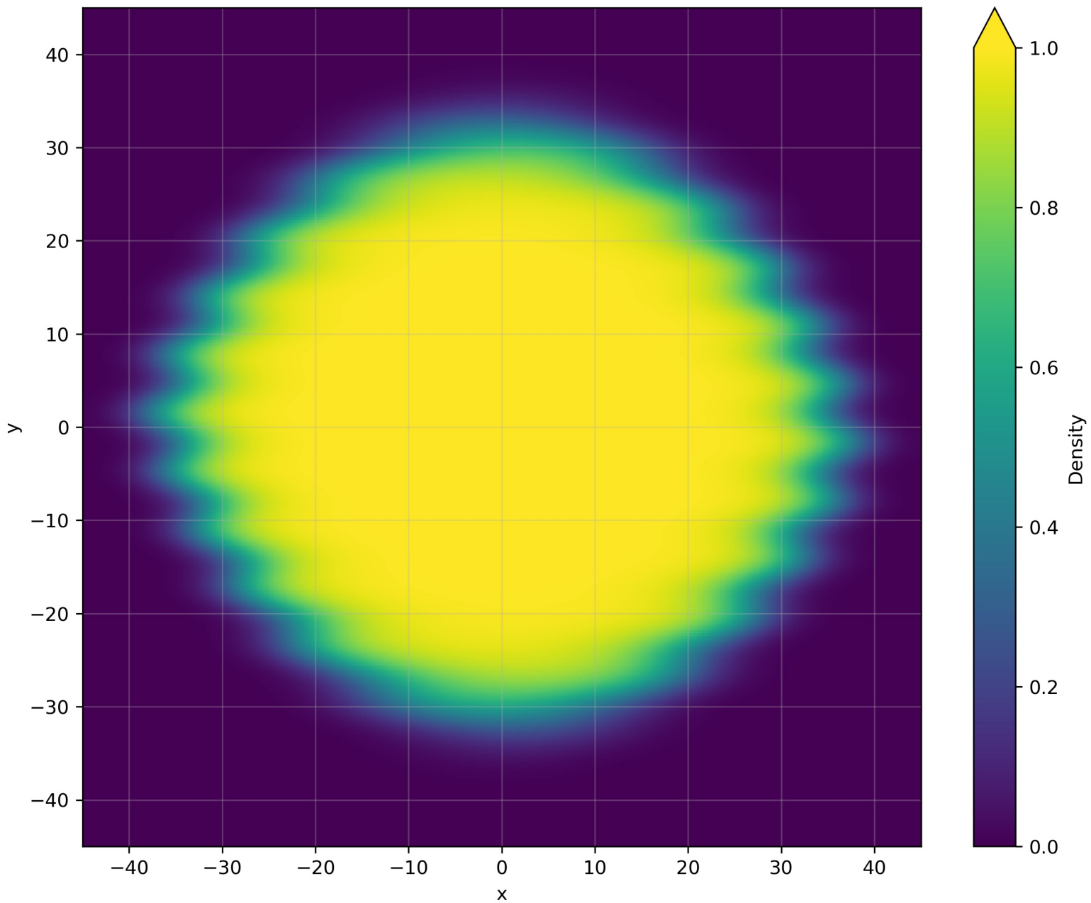
FDM of shear flow at t = 20
