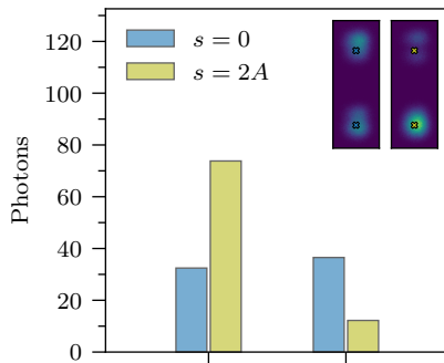
PM-SPADE
