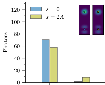
HG-SPADE
