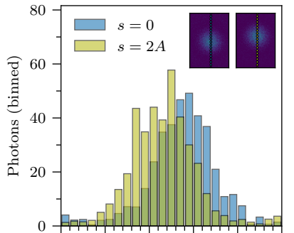
Direct imaging
