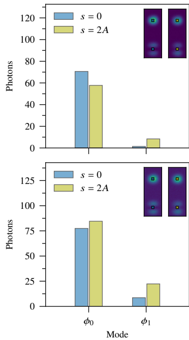
HG-SPADE (two-modes)
