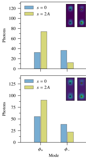
PM-SPADE
