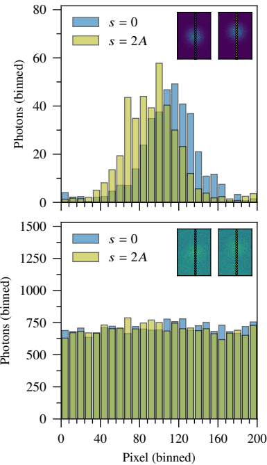
Direct imaging
