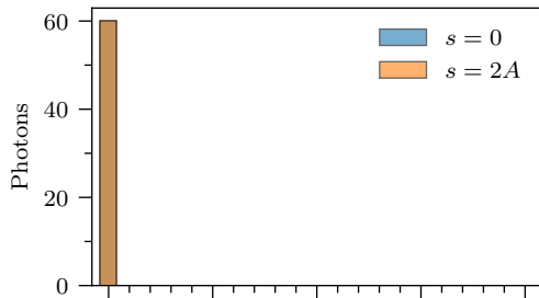
HG-SPADE ( A = 0.01\sigma )
