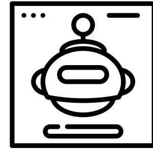
Video Generation
