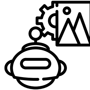
Image Generation
