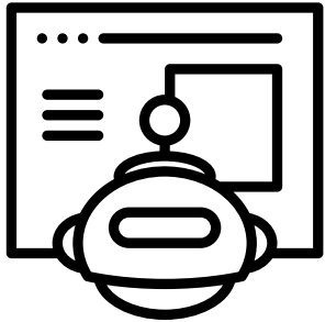
Text Generation
