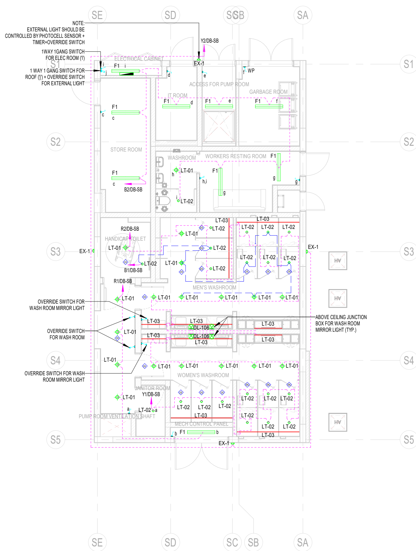
2 01-GROUND FLOOR SERVICE BLOCK LIGHTING 1 : 100
