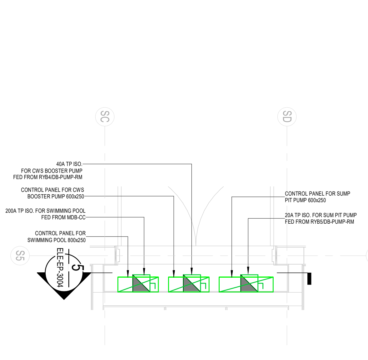
PUMP ROOM ELE.CABINET DETAILS
