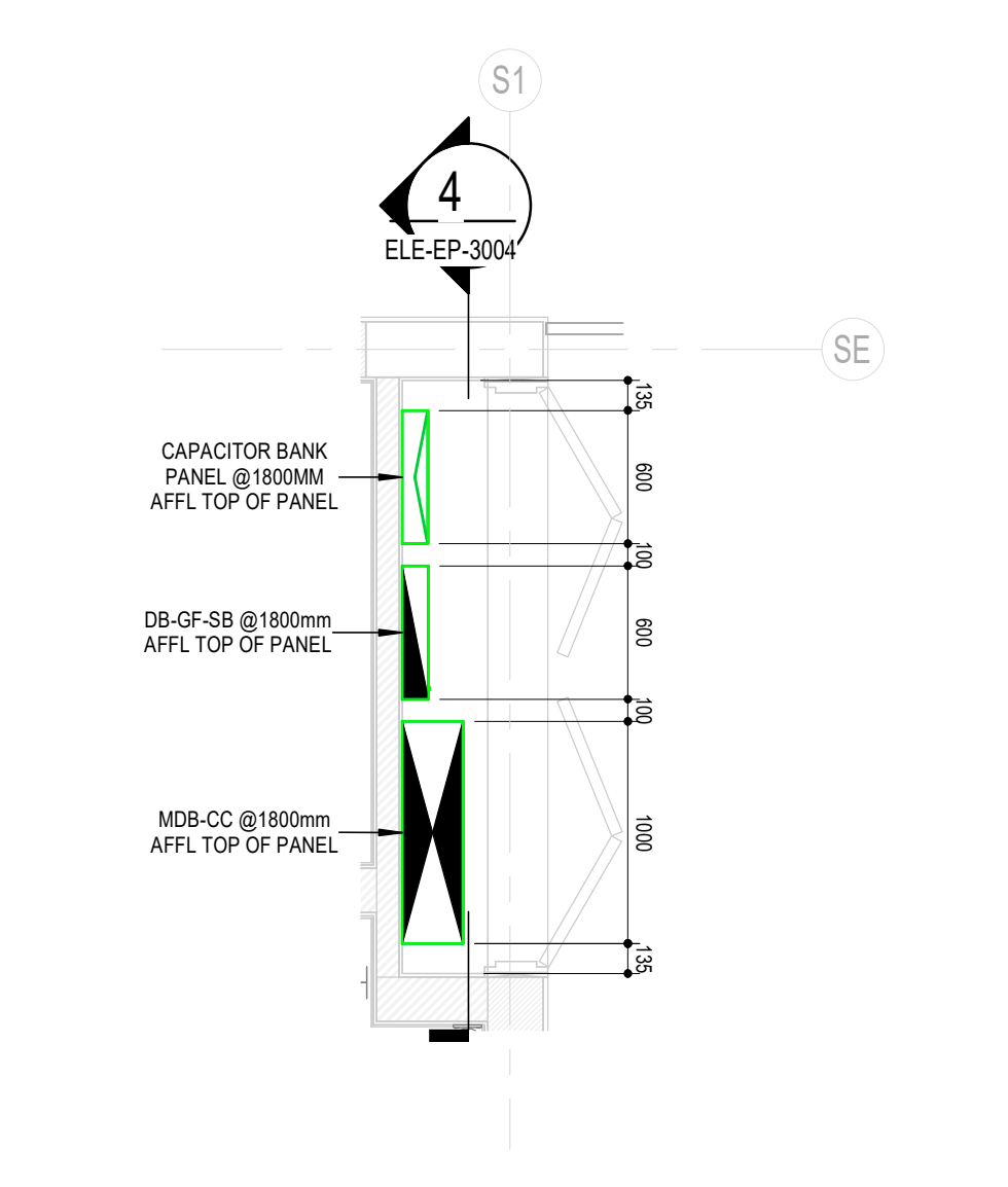
SERVICE BLOCK ELE.CABINET DETAILS
