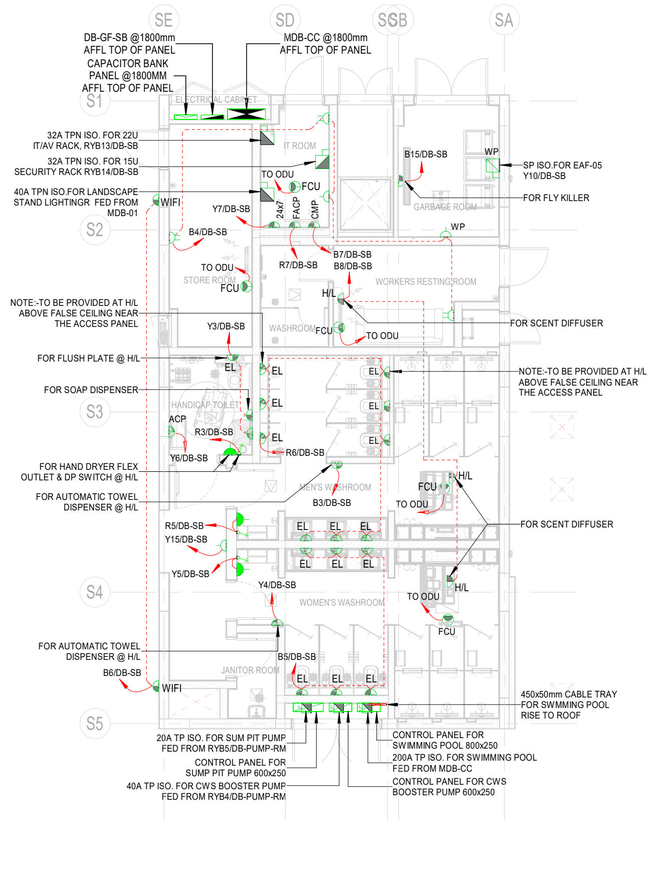
2 01-GROUND FLOOR SERVICE BLOCK POWER 1 : 100
