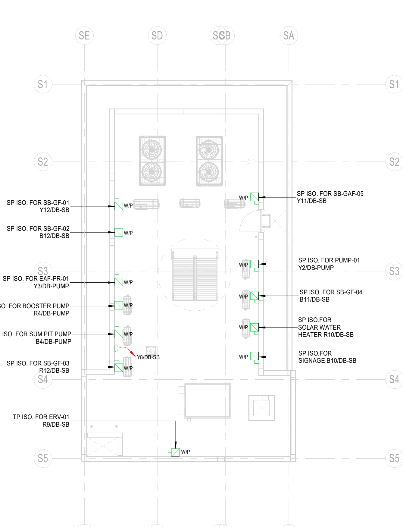
3 02-ROOF SERVICE BLOCK POWER 1 : 100
