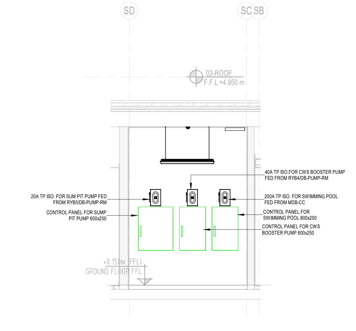
5 PUMP ROOM ELE.CABINET DETAILS SECTION 1 : 50
