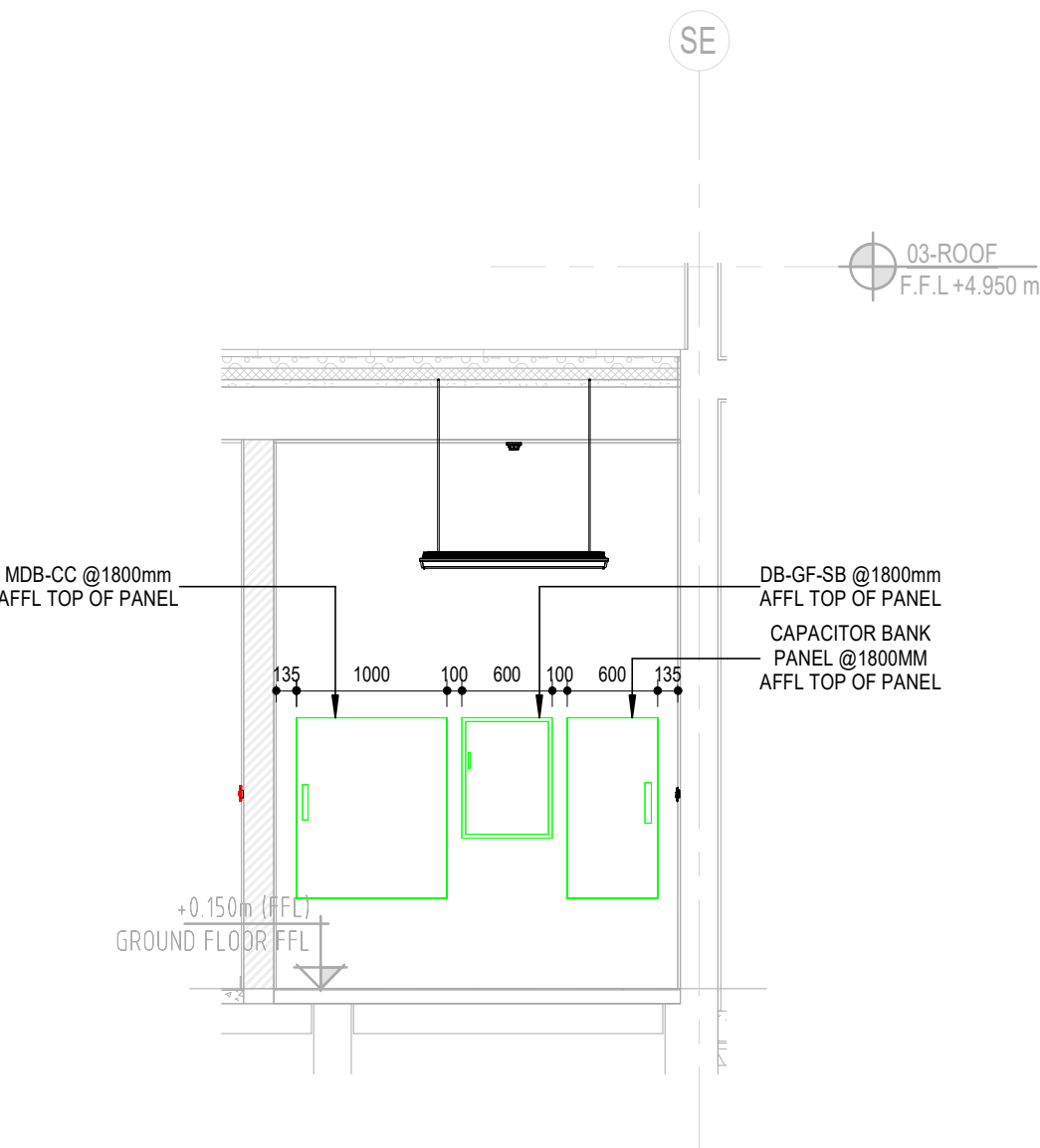
4 ELE.CABINET DETAILS SECTION 1 : 50
