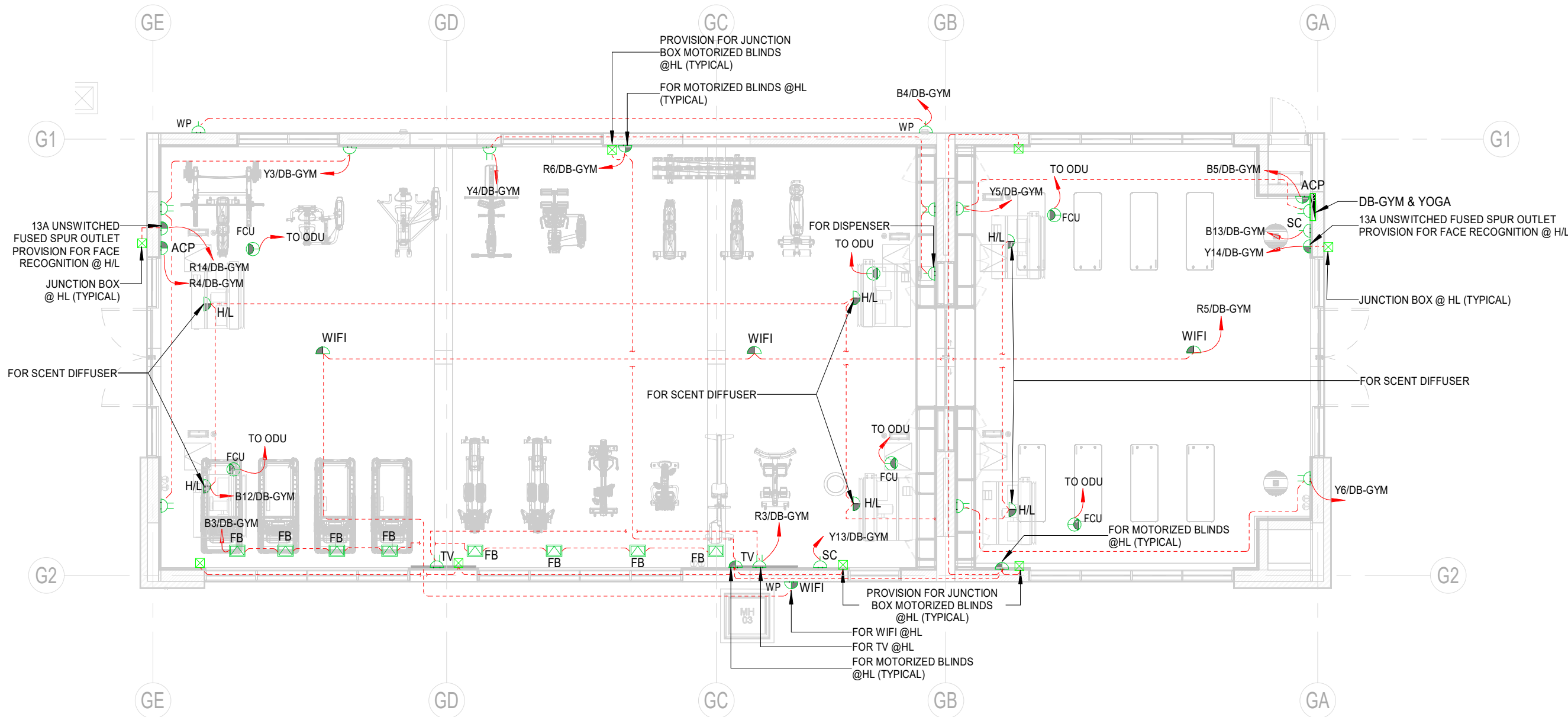
1 01-GROUND FLOOR GYM POWER 1 : 100
