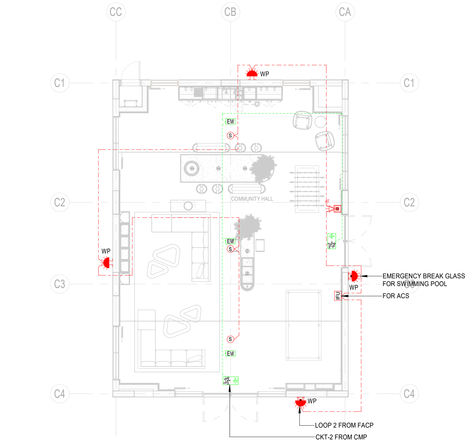
1 01-GROUND FLOOR COMMUNITY FIRE ALARM & EMERGENCY 1 : 100
