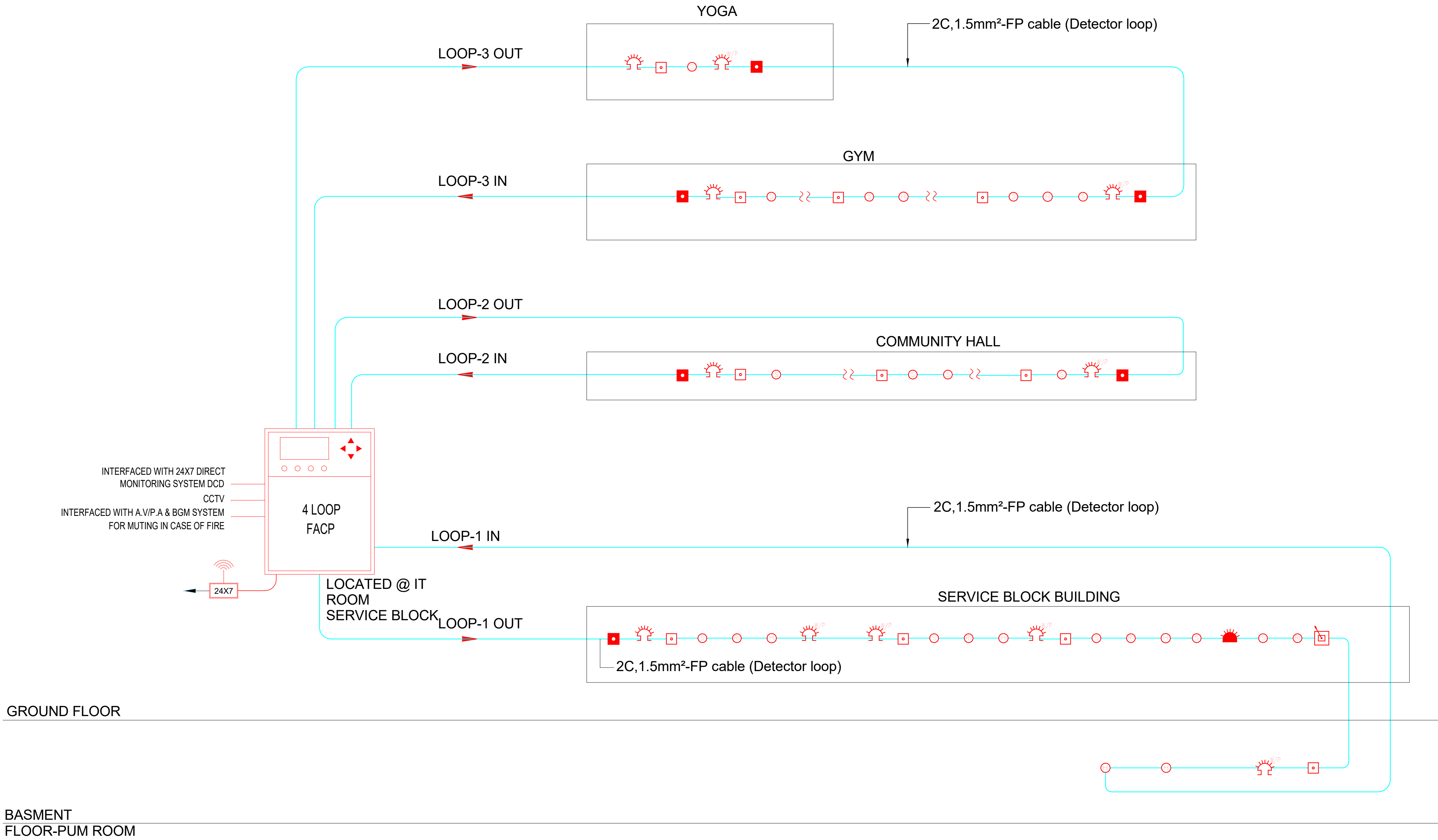
FIRE ALARM SCHEMATIC DIAGRAM
